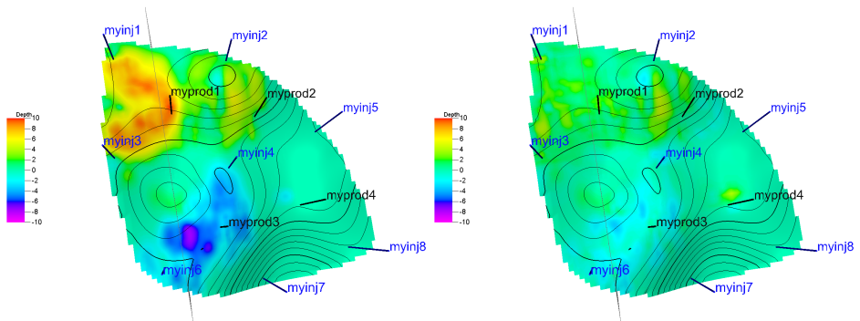
Figure 5.8: Prior (left) and updated (right) residual maps for experiment #1. Colors represent the residuals in m. Contour lines indicate the true bottom depth (without scale).
