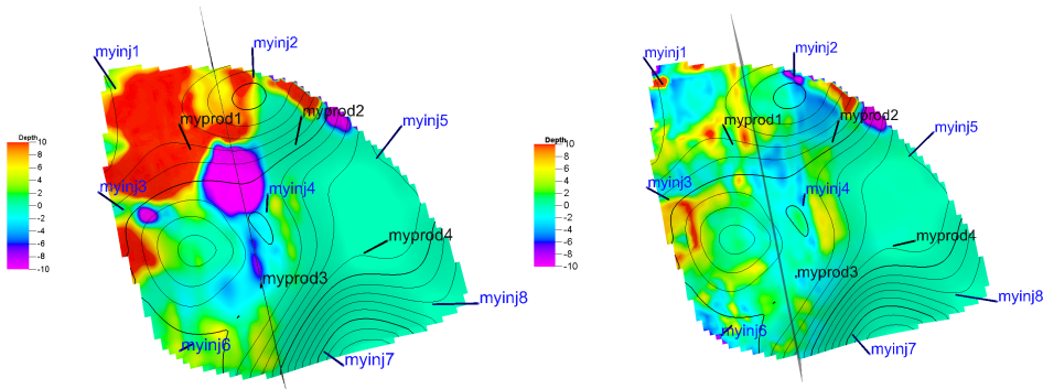
Figure 5.14: Prior (left) and updated (right) residual maps for experiment #3. Colors represent the residuals in m. Contour lines indicate the true bottom depth (without scale).
