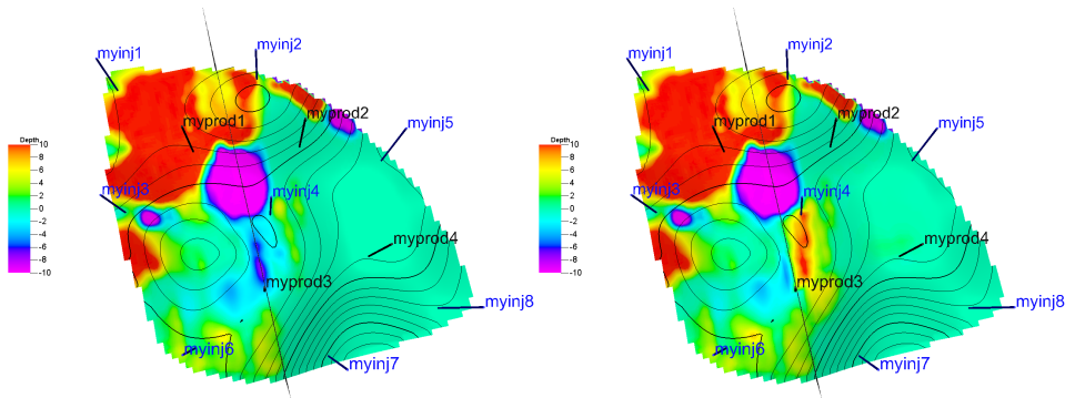
Figure 5.11: Prior (left) and updated (right) residual maps for experiment #2. Colors represent the residuals in m. Contour lines indicate the true bottom depth (without scale).
