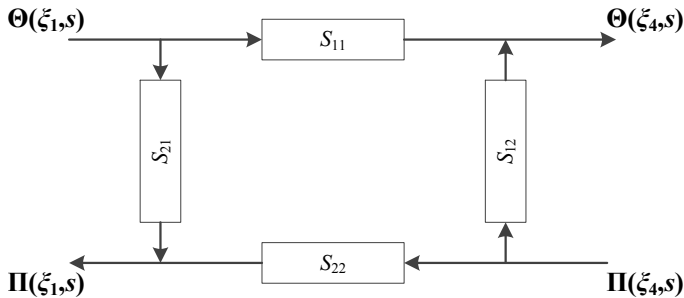
Figure 4.8: Modified block diagram representation for the model depicted in Figure 4.6.
