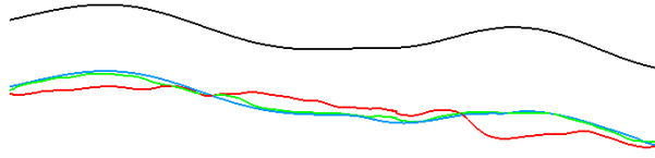
Figure 5.13: Cross section through the bottom layer of the reservoir for experiment #3. Blue represents the truth, red represents prior #2, and green represents the updated model.
