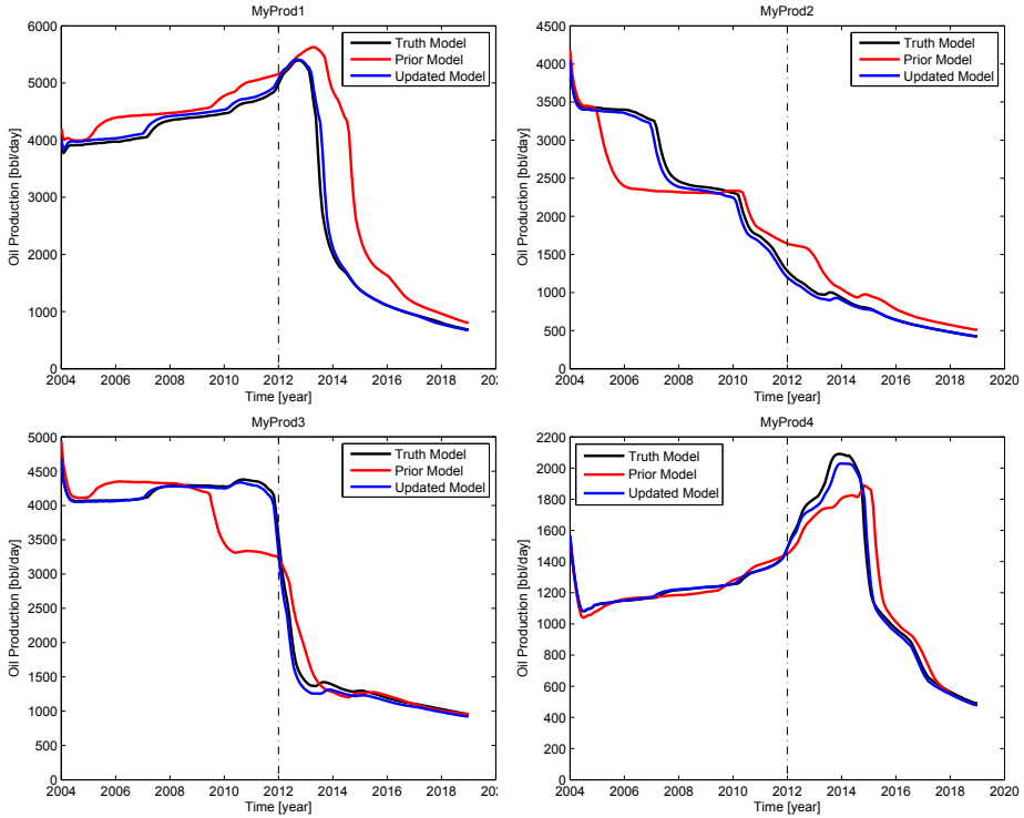
Figure 5.15: Oil flow rates of each of the four production wells for experiment #3. Red curves represent the rates of the prior model simulation, blue curves represent the rates of the updated model, and black curves represent the true rates. The vertical dashed line indicates the moment that the history match is performed.
