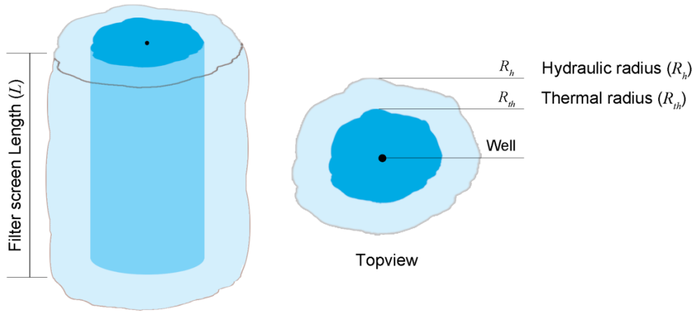
Figure 3, Simplified presentation of the resulting subsurface thermal and hydrological storage cylinder for an ATEs system for homogeneous aquifer conditions.
