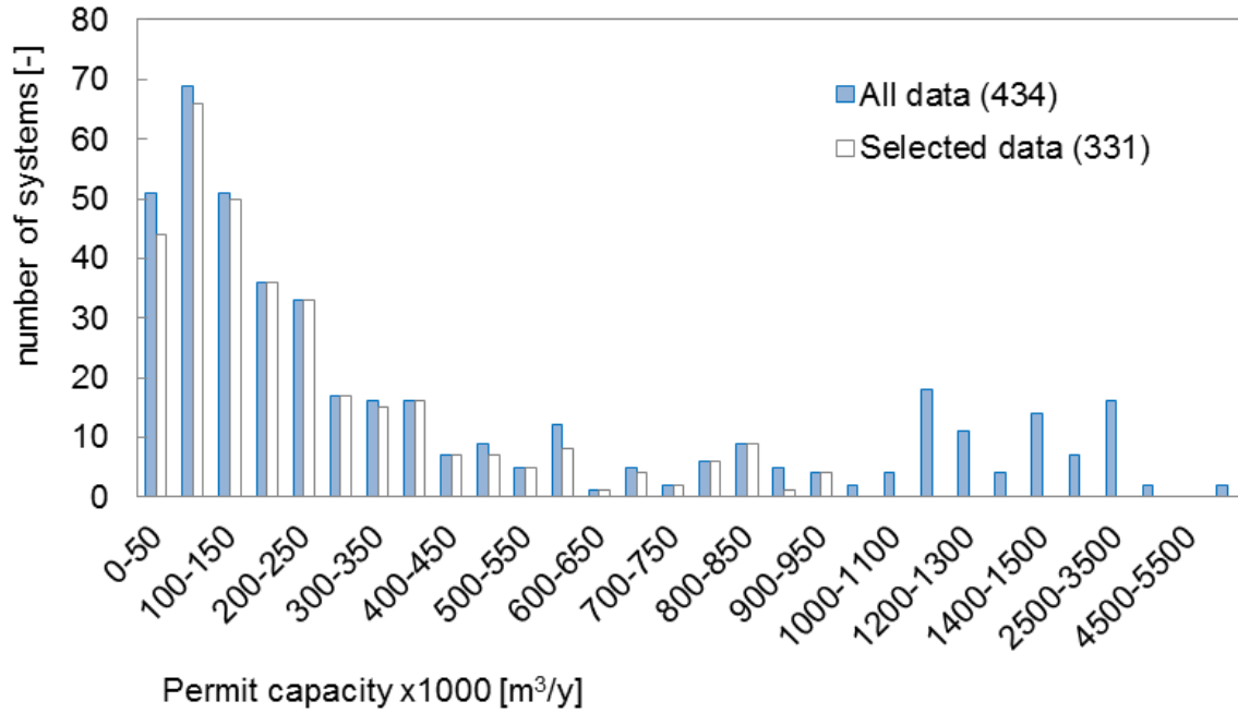
Figure 5, Frequency distribution of dataset according to permitted yearly storage volume of groundwater. Distribution of well design metrics of selected data is shown separately.
