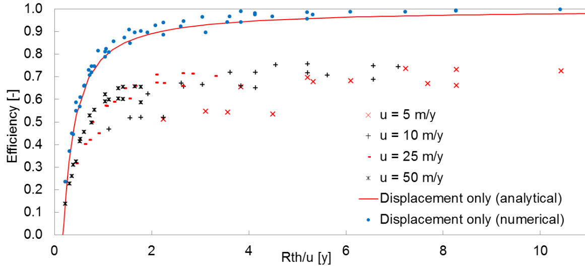
Figure 12, Relation between efficiency and thermal radius over groundwater flow velocity ( R_{th}/u ) for numerical simulation results and analytical solution (Equation (12)) for 0.5y storage period.
