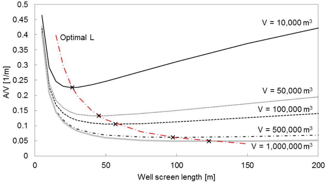
Figure 8, The A/V values for different storage volumes and well screen lengths
