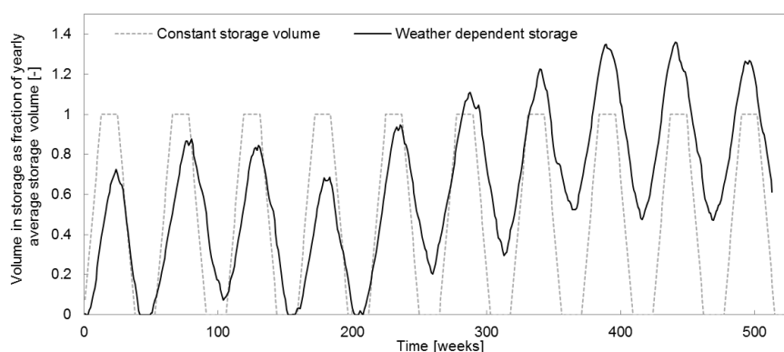
Figure 16, Volume in storage of warm well for different energy demand patterns
