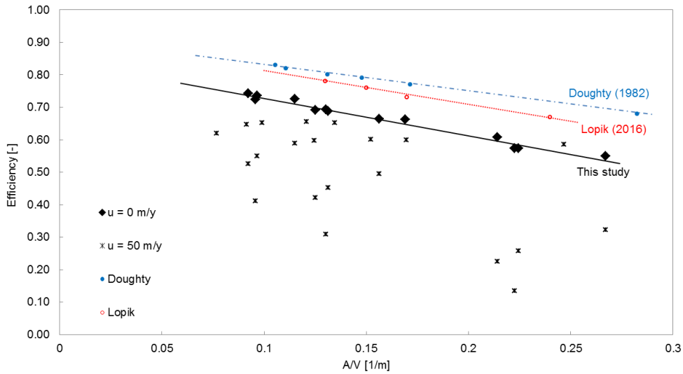
Figure 13, Simulated efficiencies relative to geometric property ( A/V ) from this and other studies at u = 0 m/y and for u=50 m/y from the simulations done in this study. The Pearson correlation between A/V and efficiency is -0,99 for u = 0 m/y. and -0.58 for u= 50 m/y. From the Lopik et al (2016) study, only the data are used from the simulations that excluded buoyancy flow.
