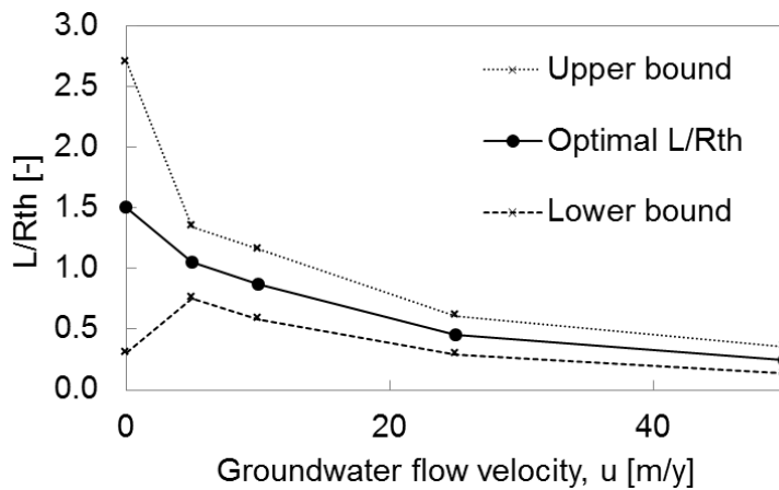
Figure 15, Optimal L/R_{th} for different groundwater flows empirically derived from simulation results
