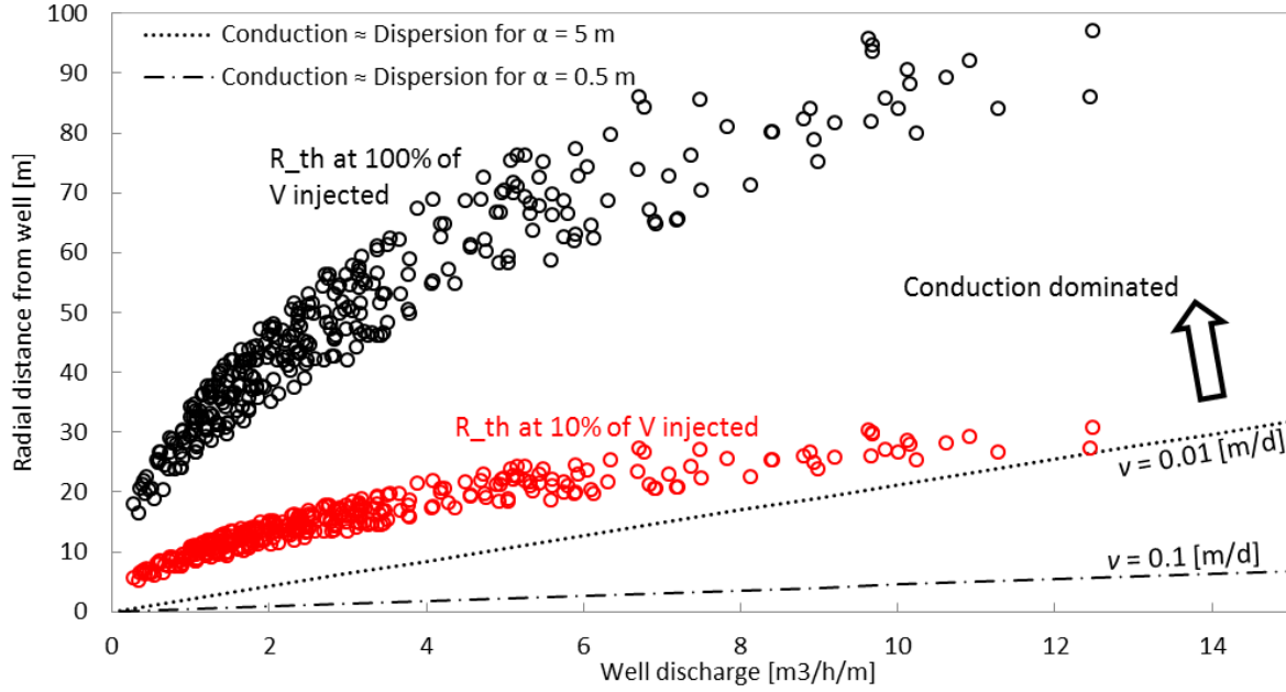
Figure 7. Lines: the relation between specific well discharge and radial distance at which the radial flow velocities where conduction and dispersion are equal (Eq. 3) for the outer-bounds of the range of thermal dispersivity regularly applied in literature. Open circles the thermal front of the ATEs systems in the data at different storage capacities related to their specific well discharge .
