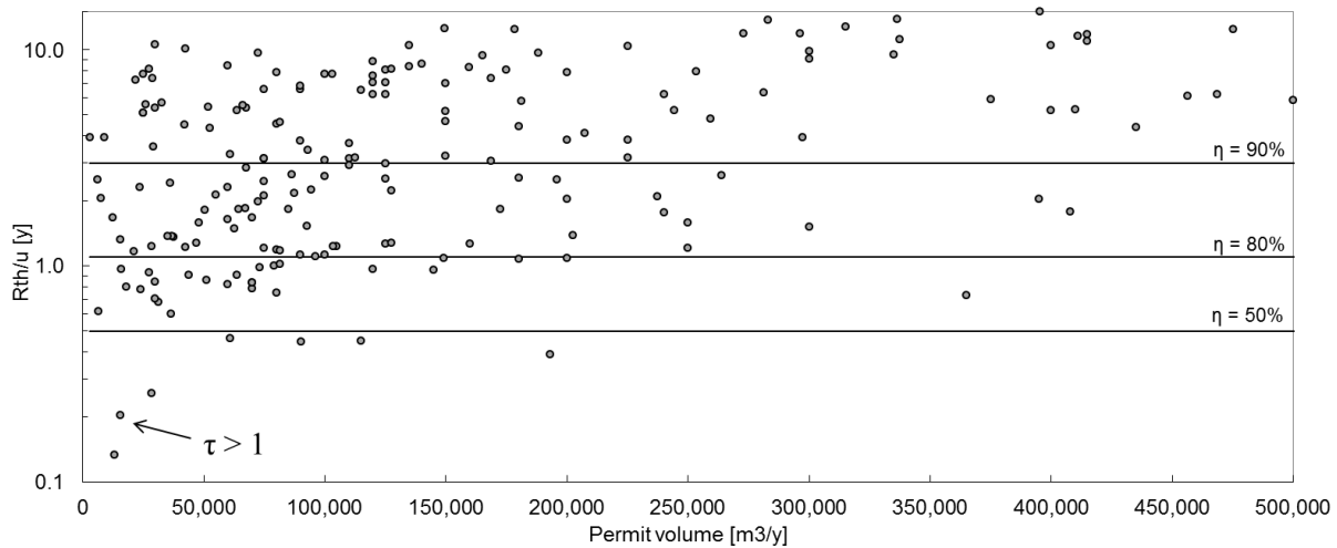
Figure 11, R_{th}/u -values for ATEs systems in the dataset with thresholds for different thermal recovery efficiencies
