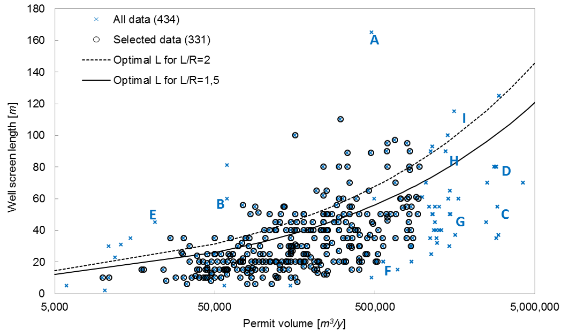
Figure 6, Dataset characteristics; outliers are excluded from the dataset. A, B=monowells with only top of upper and bottom of lower filter in the data, C=University Campus ~6 doublets, D=Office with 3 doublets, E=Office building with only extracted volume of one year available in data, unrealistically small for size of building, F=office with 4 doublets, G=Hospital with 4 doublets, H=conference center with 2 monowells, I=Office with 3 doublets
