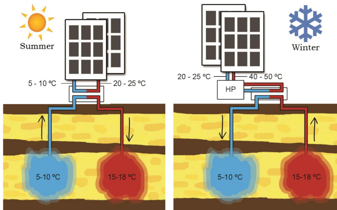
Figure 1, Illustration of the basic working principle of a low-temperature seasonal ATES system. Left: in direct cooling mode while storing heat for winter. Right: vice-versa in heating mode supported by a heat pump while storing cooling capacity for summer
