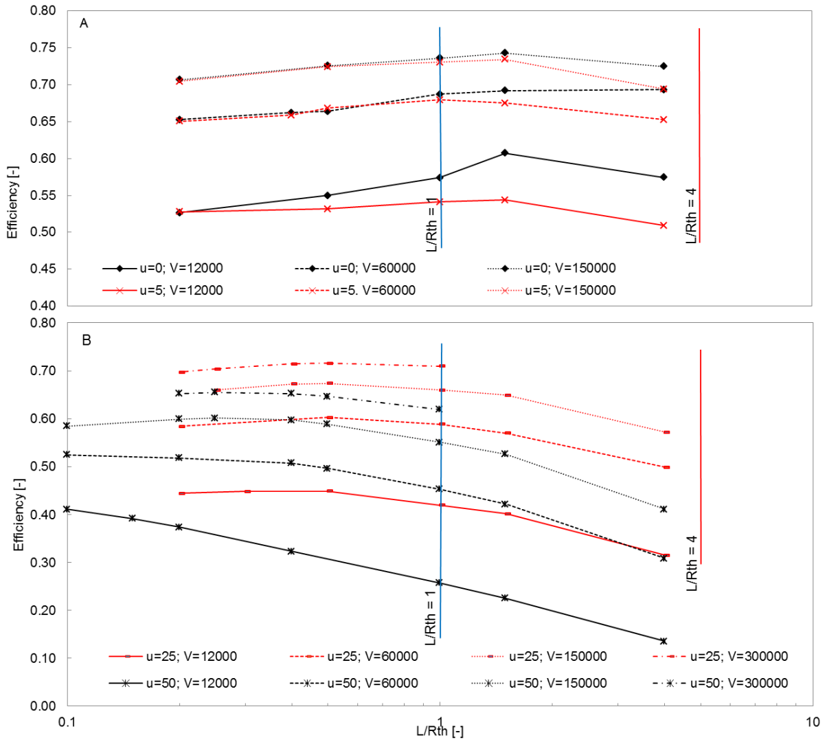
Figure 14. Simulated efficiencies for different groundwater flows ( u ) and screen length over thermal Radius ( L/R_{th} ) of various storage volumes. A. is at no/low ambient groundwater flow (Doughty applies). B. is at high ambient groundwater flow.
