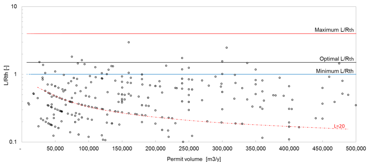
Figure 9, L/R_{th} -value relative to permit volume of ATEs systems in practice, combined with minimum ( L/R_{th} = 1 ), maximum ( L/R_{th} = 4 ) and optimal ( L/R_{th} = 1.5 ) L/R_{th} for conduction and dispersion losses
