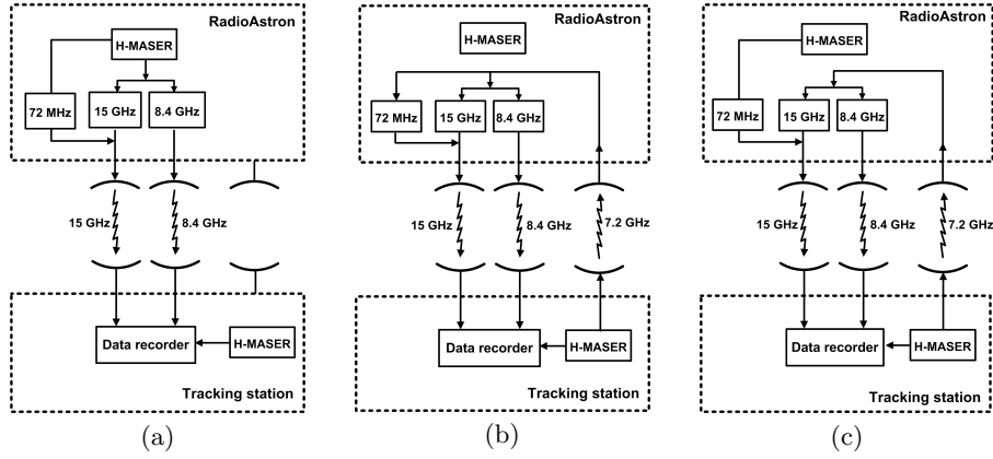
Figure 1: On-board hardware synchronization modes. (a) “H-Maser”. (b) “Coherent”. (c) “Semi-Coherent”. Note that, due to a fixed architecture of the RadioAstron on-board radio system, the 8.4 GHz tone and the carrier of the 15 GHz data link must use one and the same reference signal at any given time: either from the on-board H-maser or from the tracking station uplink.
