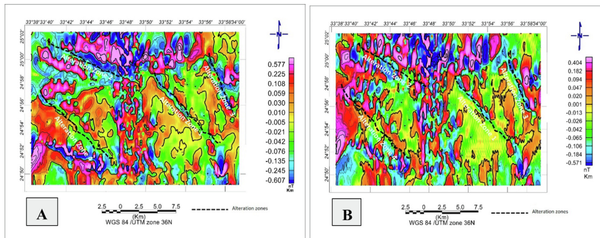
Fig. 6. (A) First vertical derivative map; (B) Total horizontal gradient aeromagnetic anomaly map of the study region.
