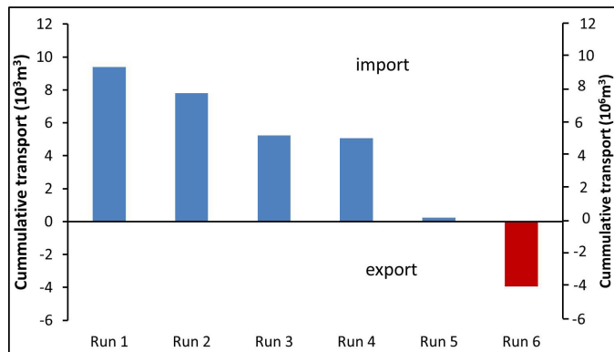
Figure 3.10: Cumulative sediment transport through the inlet for varying waves conditions and river discharges (left coordinator indicate cumulative sediment transport for first five run ( 10^3 \text{m}^3 ) and right coordinator indicate cumulative sediment transport in flood event (run 6, 10^6 \text{m}^3 ).
