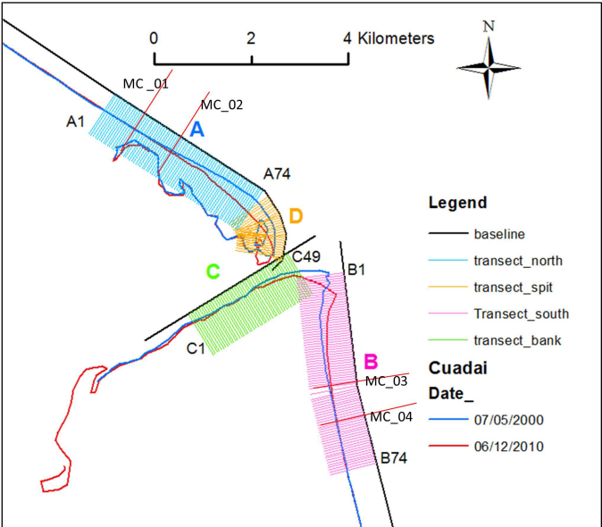
Figure 2.6: Transects at the northern side, the southern side, the riverbank and the spit created with a 50-m interval to extract shoreline changes around Cua Dai inlet.
