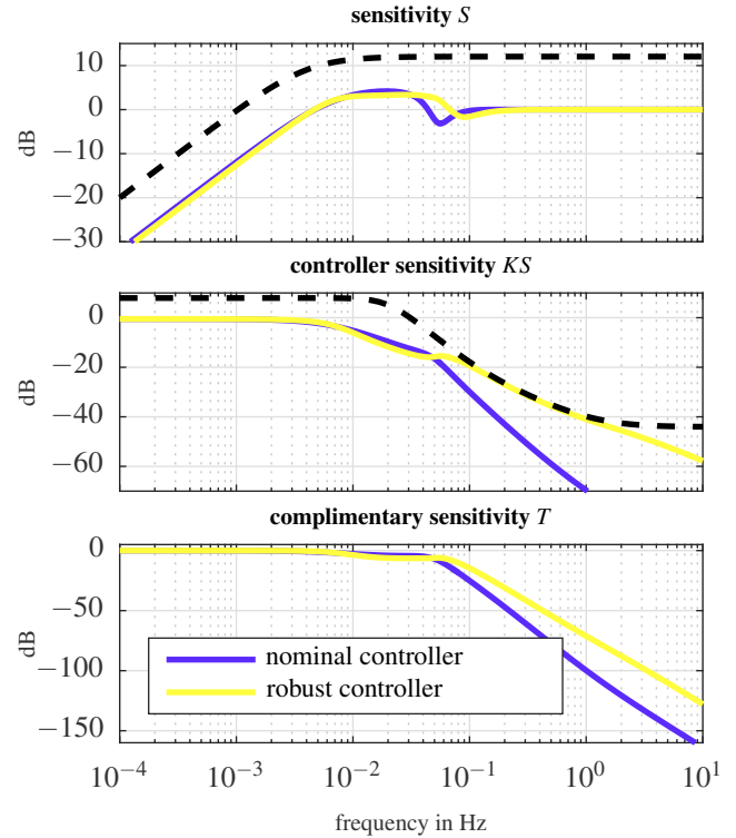
Fig. 8: Comparison between the controller performances of the nominal \mathcal{H}_\infty controller and the robust \mathcal{H}_\infty controller.
