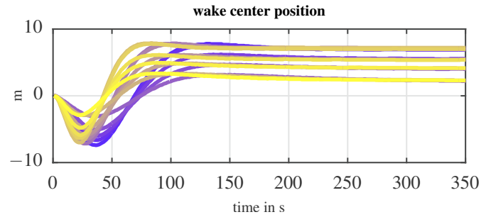
Fig. 3: A comparison of the step response simulation results of three different wind speeds, 6 m/s, 8 m/s, and 10 m/s, and within each wind speed simulation five \Delta 5 deg steps from 0 deg to 25 deg are applied by the yaw actuator. The wake center is estimated in a downwind distance of 2.5 times the rotor diameter. The steady state is removed to compare the dynamics and the final steady state. The coloring starts at dark blue for the step results at 6 m/s and ends with yellow with the last step response at 10 m/s.
