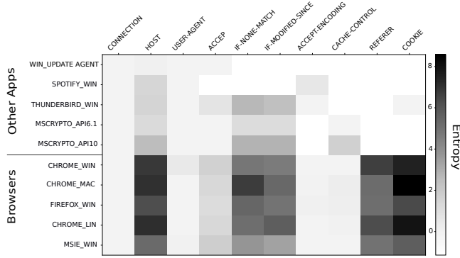
Figure 2: Heatmap representing the entropy of header values for 10 popular HTTP header and 10 different applications, including five different browsers. White cells, where entropy is equal -1, mean that the header has never been used by the application. When entropy is equal 0, it means the application uses a constant value for the header.
