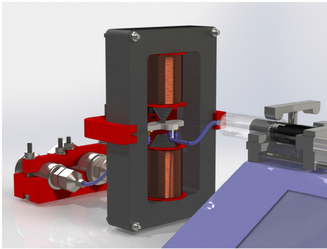
Figure 20. Test setup.
