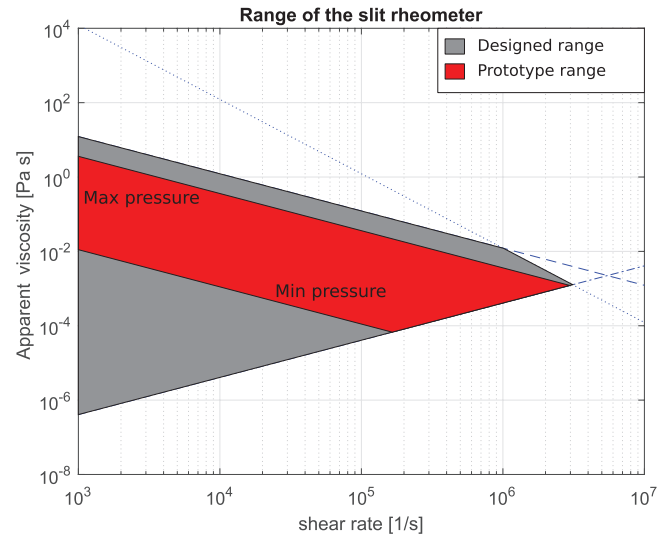
Figure 11. Prototype working range limited due to used syringe pump pressure limits.
