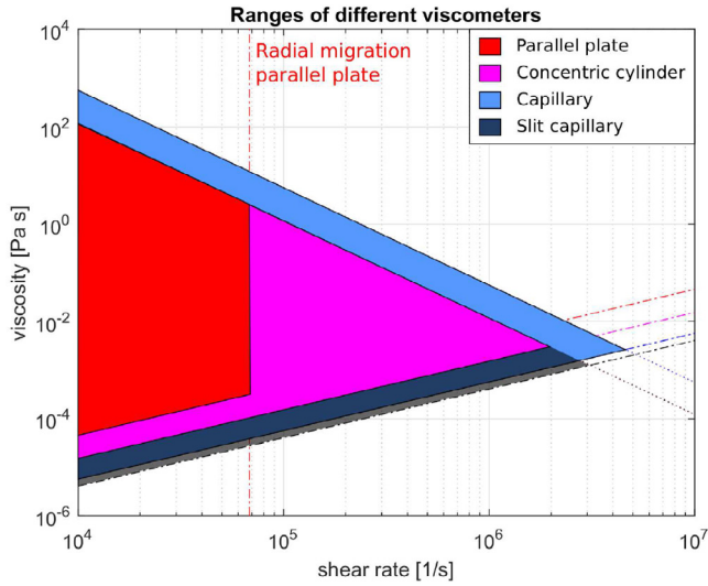
Figure 5. Theoretical ranges of the measurement principles for a gap of 35 \mu\text{m} .
