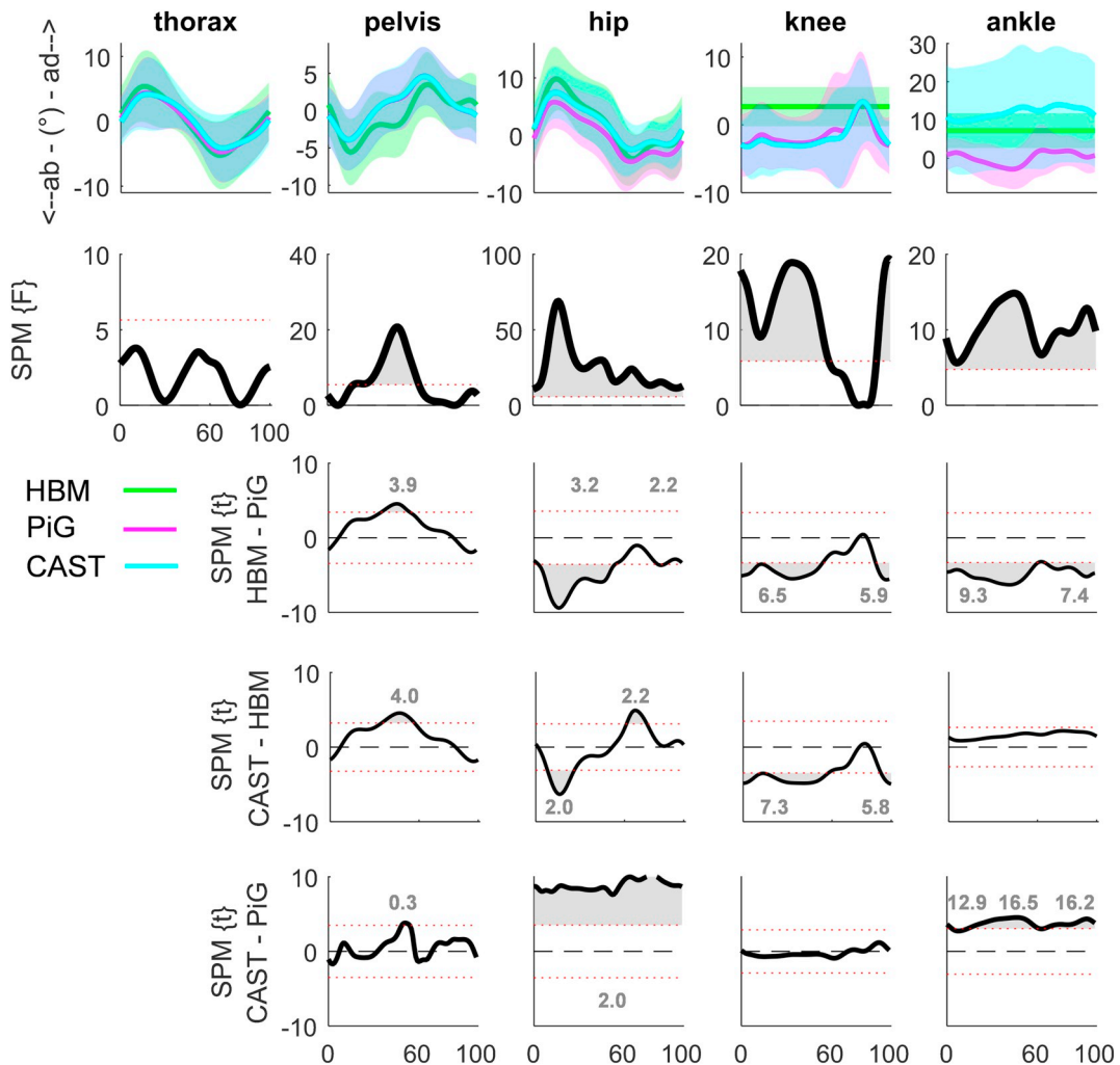
Fig. 3. Frontal plane angles. Representation of the graphs is similar as described for Fig. 2. HBM knee and ankle angles are constraint to zero degrees movement in the frontal plane. The horizontal lines represent the static values for ab-/adduction.
