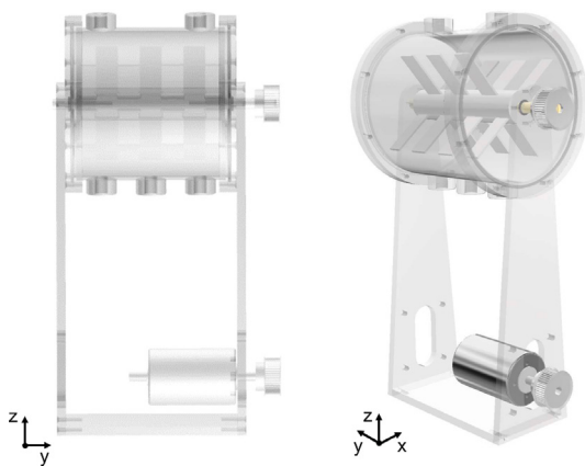
Fig. A.1. Schematic representation of the laboratory-scale horizontal stirred bed reactor. The x-y-z origin is defined in the center of the HSBR cylinder.
