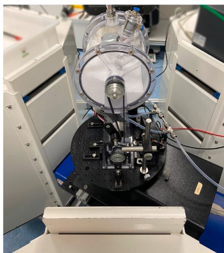
Fig. 4. Photograph of the experimental setup. The HSBR loaded with PP powder is positioned in the center of the RPT setup, comprising three \gamma -radiation detectors.
