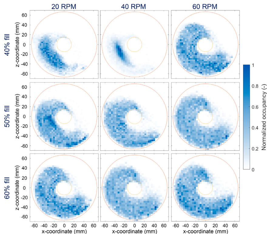
Fig. 10. Influence of the fill level and rotation speed on the tracer particle normalized radial occupancy. In each plot, the HSBR shaft is indicated by the yellow outlined circle.
