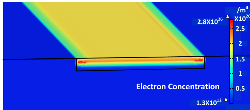
Fig. 4. Electron concentration in the \text{N}^+ region of the photodiode structure at 0 V bias condition.
