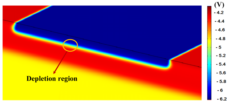
Fig. 5. Electric potential calculated from the vacuum level on a \text{P}^+ stripe to show where in the depletion region generation occurs.
