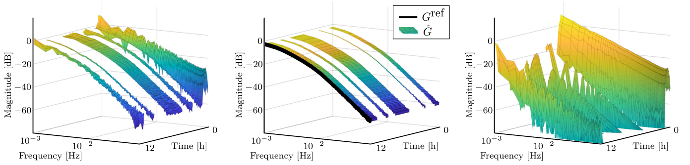
Fig. 11. Frequency–time plane results using the TIE for p = 2 . Left: transforms z^m[v] for samples v \in \mathcal{D} . Center: estimated FRF \hat{G} (surface) at samples v and the FRF of the reference model G^{\text{ref}} (—). Right: estimated transient \hat{T} at samples v .
