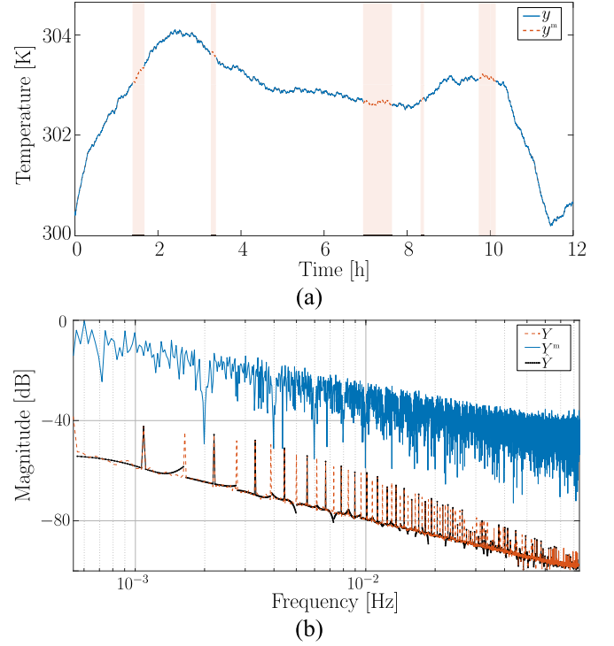
Fig. 10. Time- and frequency-domain representations of the responses of the experimental setup with and without missing samples. (a) Temperature response y (—) and the mimicked incomplete signal y^m (---). Note that the signals largely overlap. The missing data parts are highlighted in red. (b) DFT Y (---) of the complete data record and DFT Y^m (—) of the incomplete record. The locally missing samples in the time domain have a global effect in the frequency domain. Using the TIE with p = 2 , the estimate \hat{Y} = \hat{K} \hat{\Theta} (—) accurately approximates Y (---) at and around the odd EF lines while having access to Y^m only (—).
