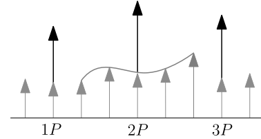
Fig. 4. Frequency-domain representation of response Y in (4) for N_Y = 0 , P = 3 , and \gamma = 1 . At the EF lines [1P, 2P, 3P] , the response consists of both the transient (gray arrows) and the periodic response (black arrows). At the NEF lines, the response contains only transient contributions. The gray line represents the local transient estimate based on the n_r frequency lines around the 2P th EF line.
