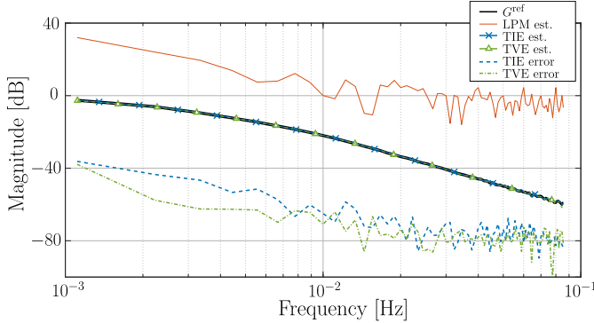
Fig. 12. Bode magnitude plot of the reference model G^{\text{ref}} (—), and the estimates obtained from the classical LPM (—), the TIE (*), and the TVE ( \Delta ) for p = 2 . In addition, the model errors of the TIE (—) and TVE (—) are shown (—). Both the TIE and TVE achieve accurate identification from incomplete data, in contrast to the classical LPM.
