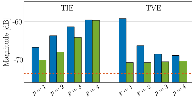
Fig. 13. Model errors e_{\text{TIE}}^{[p]} and e_{\text{TVE}}^{[p]} (■) and the estimated contributions due to stochastic noise (■).
