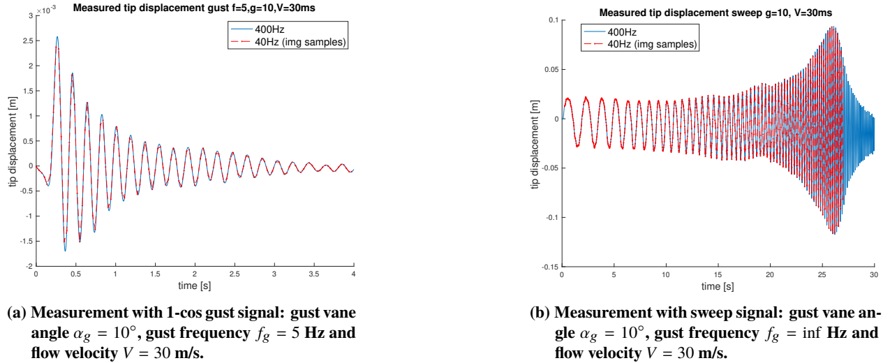
Figure 8 Spline model of the laser measured (400 Hz) tip displacement of marker ID[1] sampled at capture intervals of Cam1 ( \approx 40 Hz). From runs with discrete gust and sweep signals.
