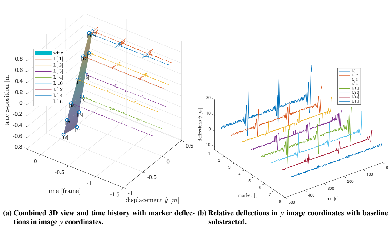
Figure 10 Time series of marker- y deflections in the image coordinates across 498 image sequences, as a result of gust excitations from run R1.
