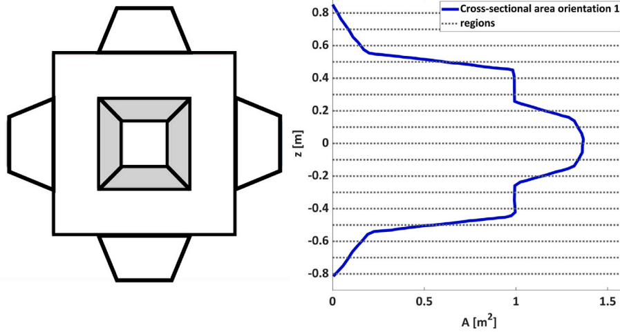
Fig. 3. Sample solidity curve distribution for one of the Cubipod orientations with 22.5^\circ increments.
