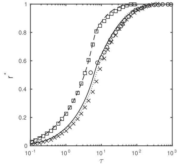
Fig. 13. Dimensionless contact radius r^* with dimensionless time \tau for Dynamic contact angle: present without IBM (—), present with IBM (×), experiments by Lavi and Marmur (2004) (○), simulations by Legendre and Maglio (2015) (···) and Static contact angle: present without IBM (—), present with IBM (□).
