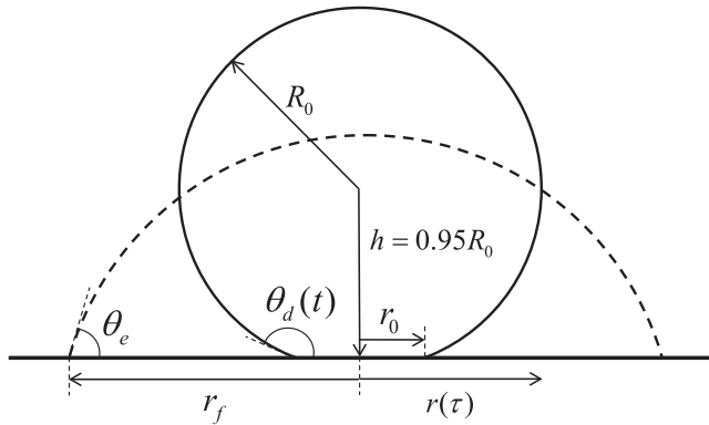
Fig. 12. Schematic representation of the initial (—) and equilibrium (---) states of the a droplet spreading on a flat surface with dynamic contact angle.
