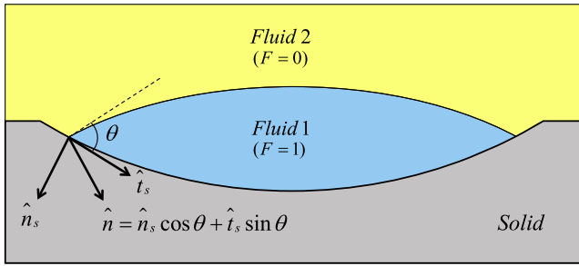
Fig. 3. Contact angle boundary condition implementation at solid boundaries. The fluid-fluid-solid contact line runs perpendicular to this figure.
