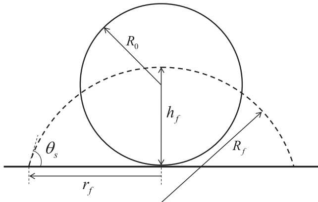
Fig. 4. Schematic representation of the initial (–) and equilibrium (– –) shapes of the droplet on a flat surface with static contact angle without gravity ( Eu = 0 ).
