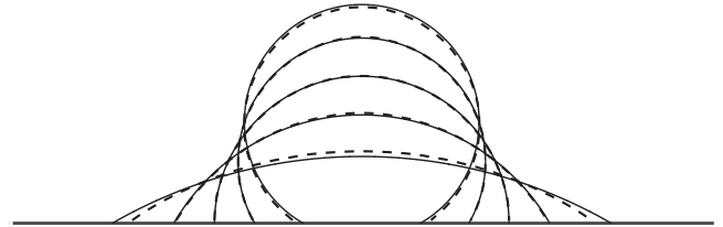
Fig. 6. Analytical (–) and numerical (– –) equilibrium droplet shapes on a flat surface without gravity ( Eu = 0 ) for static contact angles \theta_s = 30^\circ, 60^\circ, 90^\circ, 120^\circ and 150^\circ .
