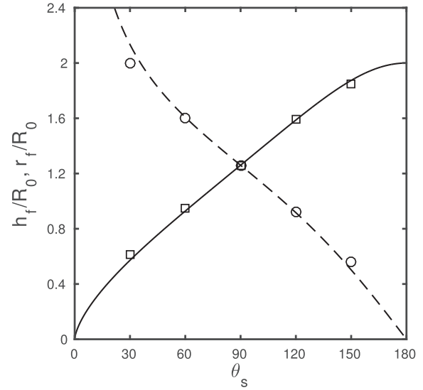
Fig. 5. Dimensionless droplet parameters for the equilibrium shape of a droplet on a flat surface without gravity ( Eu = 0 ): analytical height (–), numerical height (□), analytical contact radius (– –), numerical contact radius (○).
