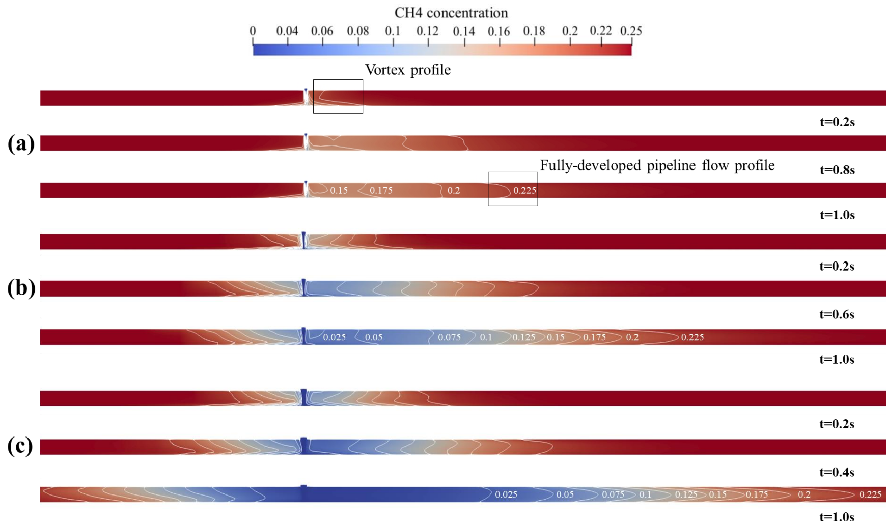
Fig. 10 CH4 concentration distribution of different leak sizes, (a) Case 1: 100mm, (b) Case 2: 200mm, (c) Case 3: 300mm.
