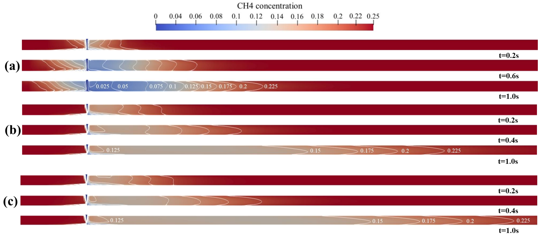
Fig. 15 CH4 concentration distribution of different leak locations, (a) Case 4: underground pipeline, (b) Case 5: vertical pipeline, (c) Case 6: above-ground pipeline.
