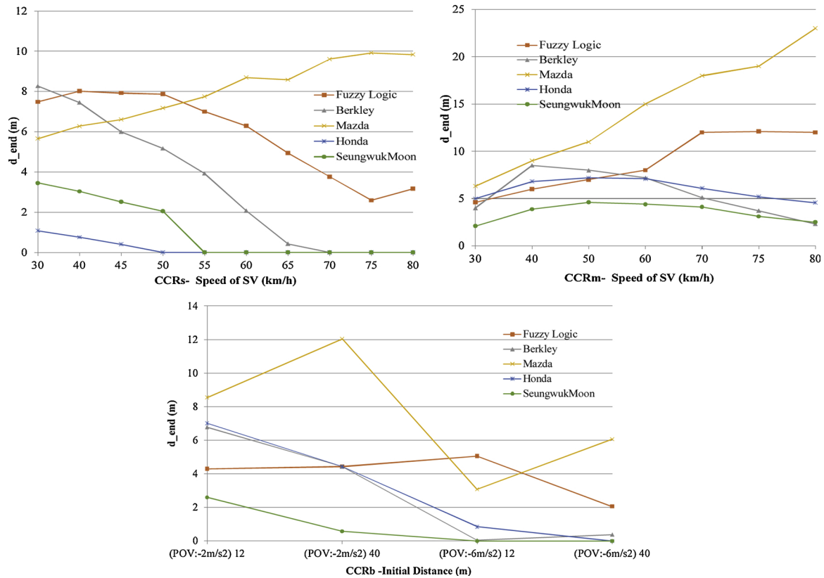
Fig. 12. Relative distances between two vehicles at the end of tests.
