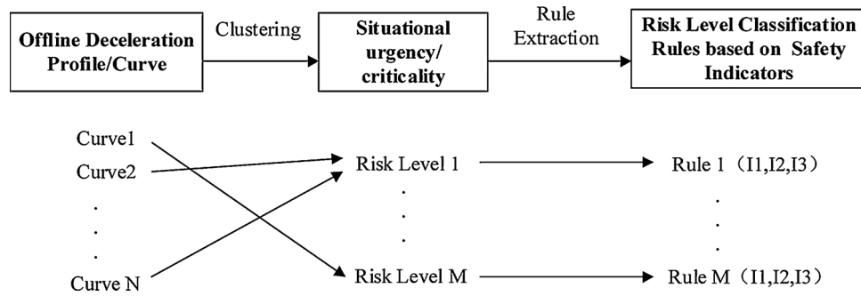
Fig. 2. Risk level classification methodology proposed in the paper.
