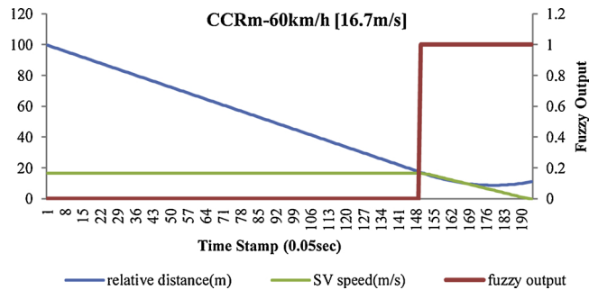
Fig. 14. Simulation history data for CCRm-60 km/h scenario.
