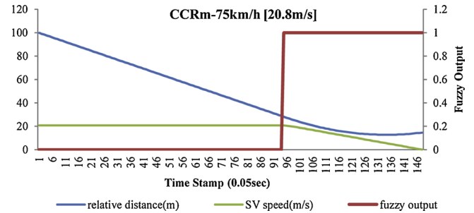
Fig. 16. Simulation history data for CCRm-75 km/h scenario.
