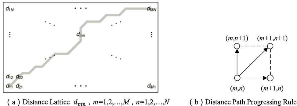
Fig. 5. Diagram of DTW distance calculation (Matlab 2018R, 2018).
