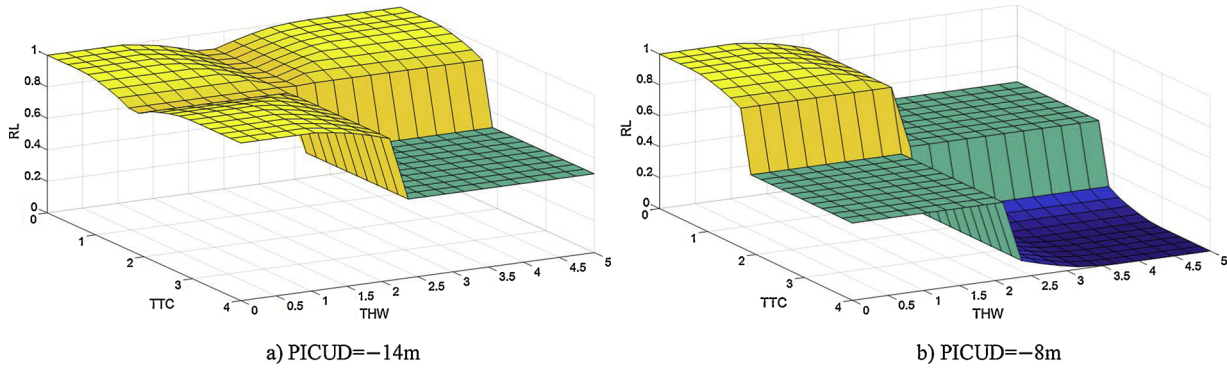
Fig. 10. Optimal fuzzy logic output surface.
