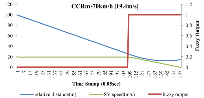
Fig. 15. Simulation history data for CCRm-70 km/h scenario.
