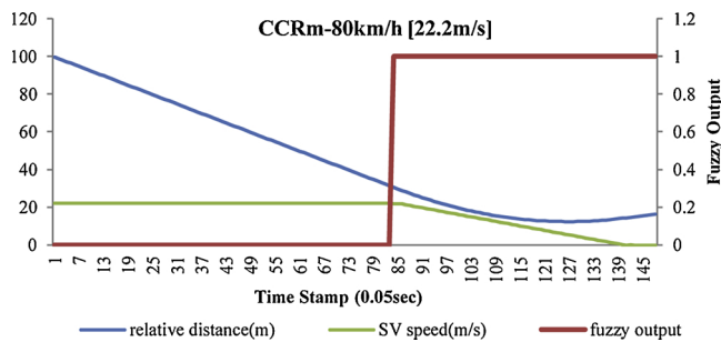
Fig. 17. Simulation history data for CCRm-80 km/h scenario.
