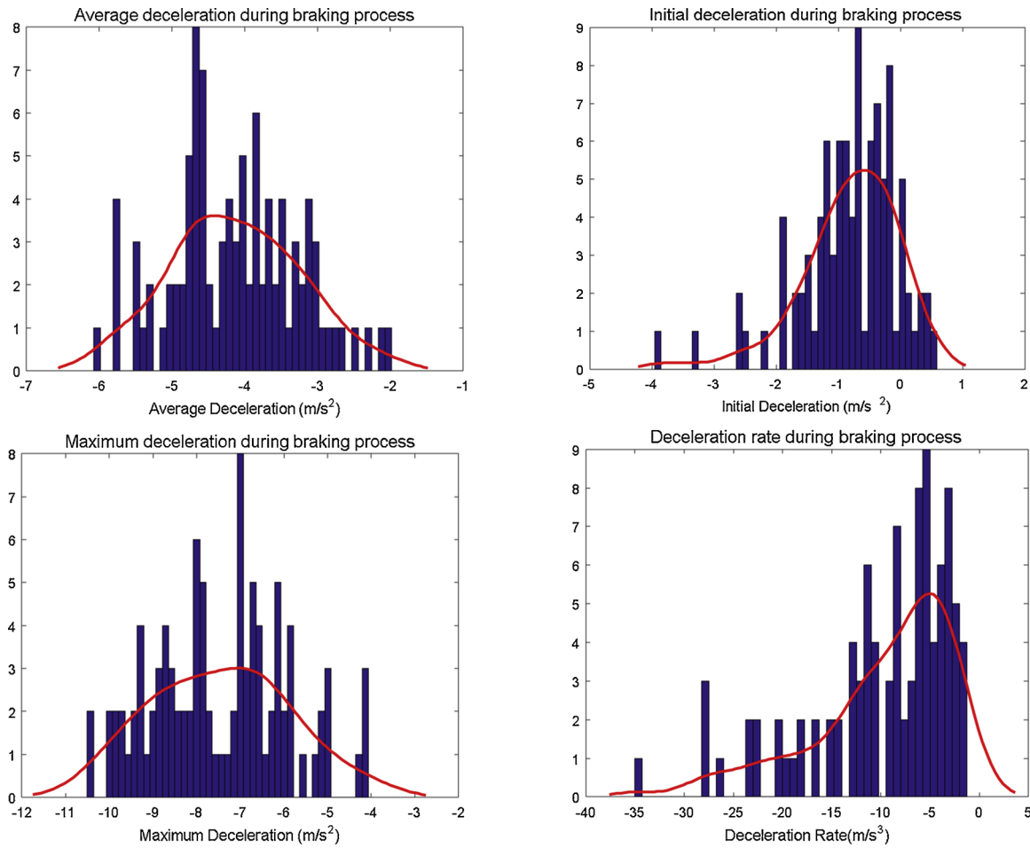
Fig. 4. Statistics of deceleration profiles extracted from “100-car” near-crashes.
