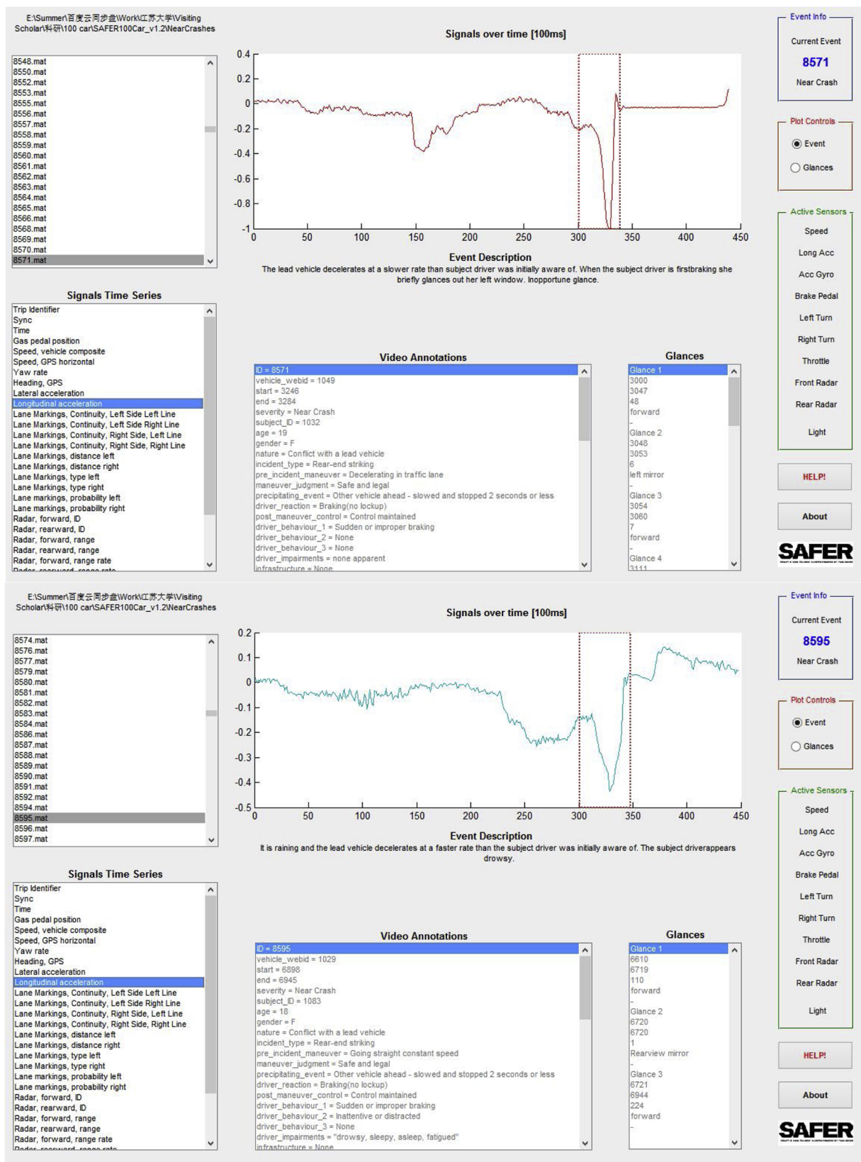
Fig. 3. Deceleration curves of sample #8571 and #8595 (deceleration started before critical event started) extracted from Natware.
