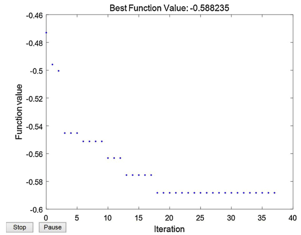
Fig. 9. PSO optimization iterative process output from Matlab.
