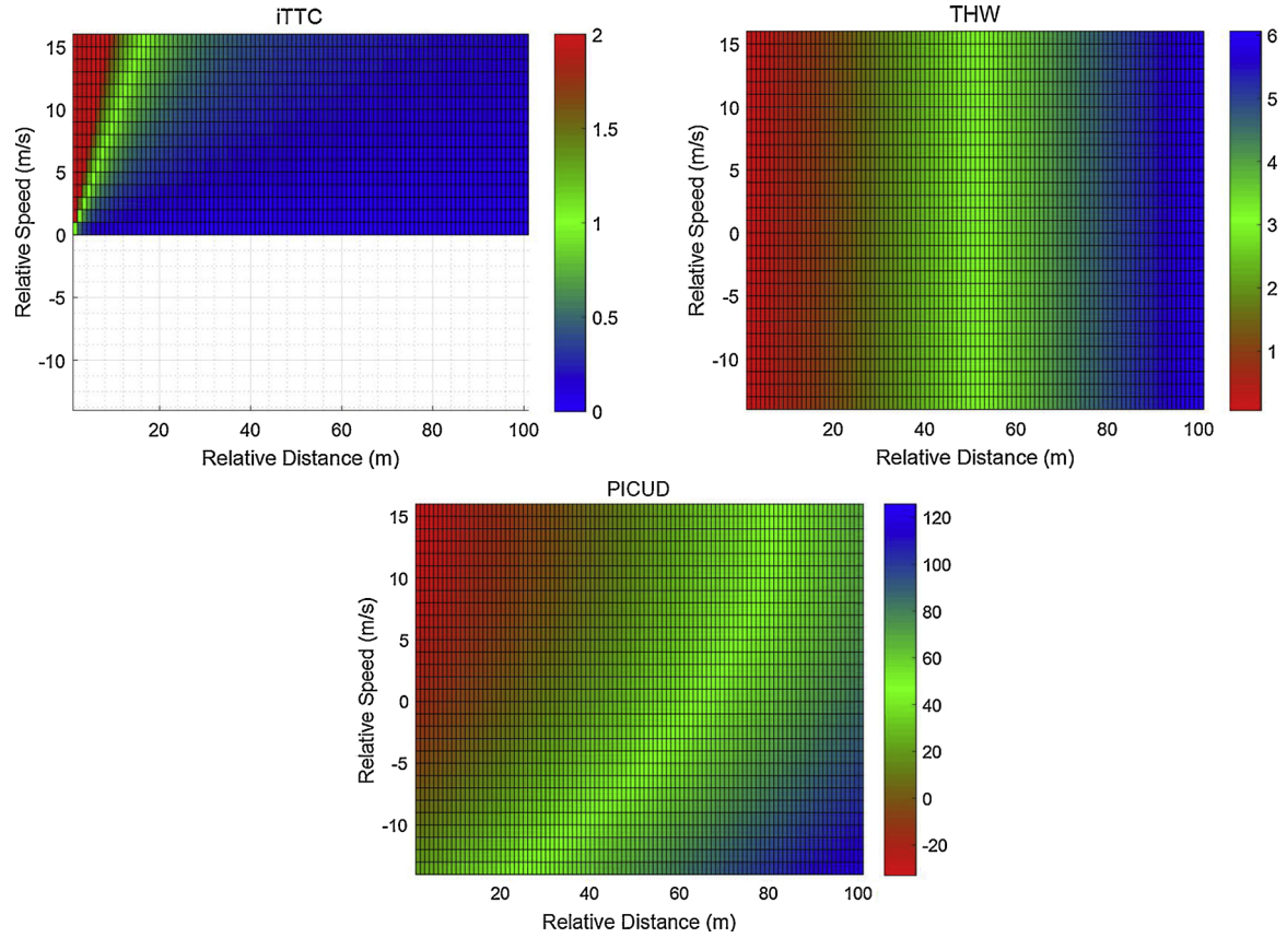
Fig. 6. Distribution of iTTC (1/s), THW (s) and PICUD (m) in relative distance-relative velocity plane (Mullakkal-Babu et al., 2017).
