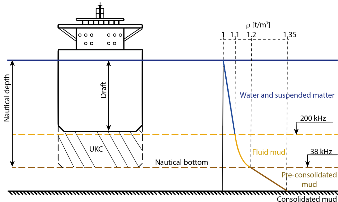
Figure 1. The nautical bottom concept at the Port of Rotterdam for the density limit of 1.2 \text{ t/m}^3 . From Kirichek et. al., 2018.
