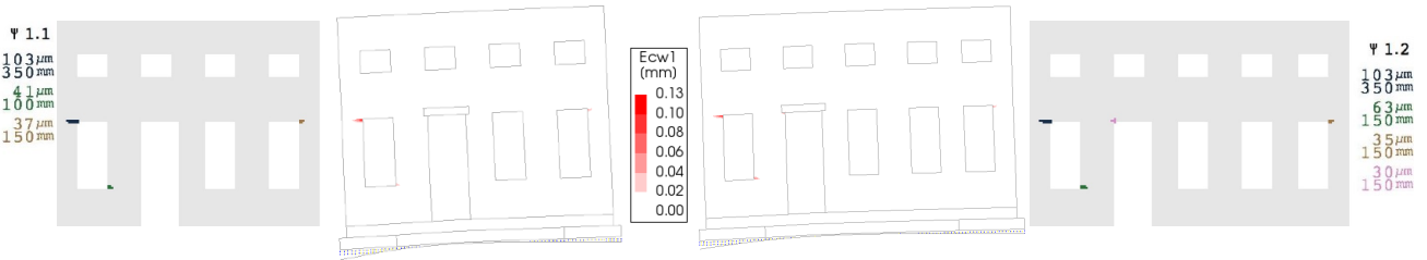
Fig. 4. Crack width (Ecwl) from the FEM model, center, for the short and long façades (left and right); and extremes, the automatically-processed damage value \Psi with interpreted crack pattern.
