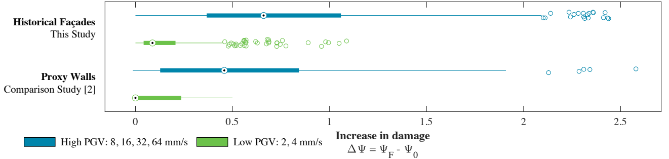
Fig. 10. Comparison between walls and historical façades only for earthquake vibrations. An increase in damage of 0.5 is visible to the naked eye. The range of parameters has been restricted for the walls so as to generate a one-to-one comparison.
