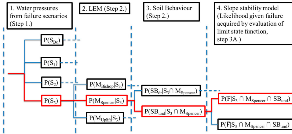
Figure 8. Presents an overview of the different combinations of scenarios and model choices. Level 1: Water pressure from failure scenarios (i.e. S_{Bc} :“Base case”, S_1 :“Saturated levee”, S_2 :“Conductive layer”, and S_3 :“Pond connection with aquifer”). Level 2: LEM (i.e. M_{Bishop} , M_{Spencer} and M_{Uplift} ). Level 3: Soil reaction behaviour (i.e. SB_{dri} : drained, and SB_{und} : undrained). Level 4: Likelihood given failure (F) and non-failure (F). Red branch contains MLC, as an example.
