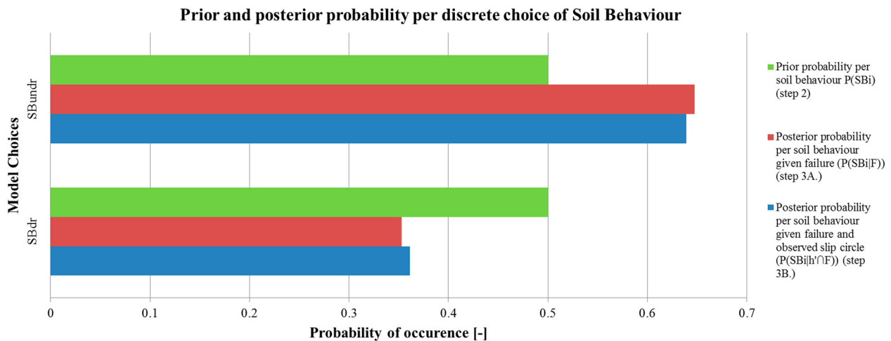
Figure 13. Prior probability per choice of soil behaviour both drained ( SB_{dr} ) and undrained ( SB_{undr} ) and equally distributed probabilities (green), the posterior probabilities per choice of soil behaviour given failure (red) and observed geometry of slip surface (blue).
