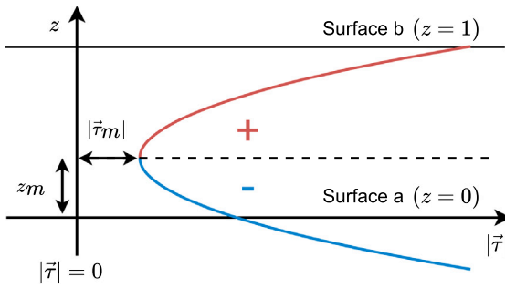
Fig. 2. A schematic representation of the shear stress magnitude |\tau| over the film height. The minimum shear stress |\tau_m| and the z -coordinate of the minimum shear stress z_m are indicated. The red part of |\tau| (above z = z_m ) corresponds to the positive solutions of Eq. (20), the blue part (below z = z_m ) corresponds to the negative solutions.
