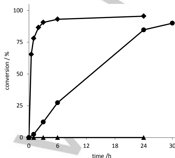
Figure 1. Time-courses of the RasADH-catalyzed reduction of butyrophenone (◆), ethyl thiobenzoate (●) and benzoic acid ethyl ester (▲) using lyophilized E. coli cells containing recombinant RasADH. Conditions: 50 mM KPi buffer (pH 7.5), (10 % v/v) 2-propanol, [NADP + ] = 1 mM, c ( E. coli ) = 20 g L -1 , c (starting material) 0 = 10 mM, T = 30°C.
