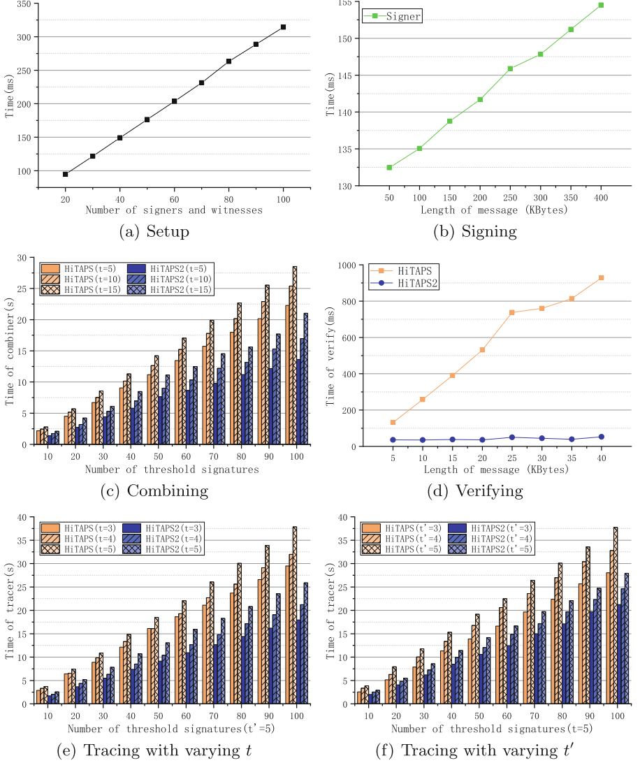
Fig. 8. Computational Costs.
