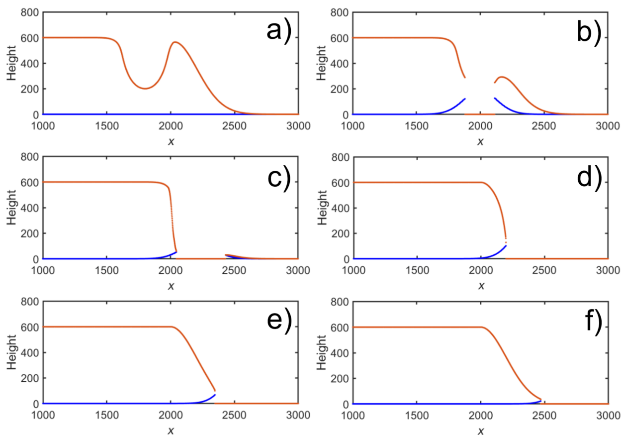
Figure 6: Simulations showing the evolution of the half-Gaussian-shaped sidewall (with \sigma = 200 ) of a deposit of height 600 as a function of the etch position. The red lines indicate the top part, as etched from above, and the blue lines the bottom part, as etched from below. In (a–f), the beam was positioned from x_0 = 1800 to x_0 = 2800 in steps of 200. All other parameters were kept constant at \sigma_d = 100 , S_d = 5 , \sigma_s = 140 , S_s = 5 , and w = 20 . The number of exposures was 80. All dimensions are in arbitrary units.
