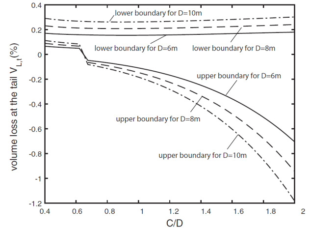
Figure 8. Volume loss at the tail when tunneling in sand
