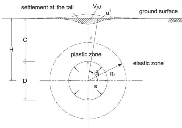
Figure 7. Deformations around a shallow tunnel at the tail
