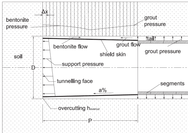
Figure 2. The range of volume loss at the tunnelling face when tunnelling with a diameter D=6 m in clay
