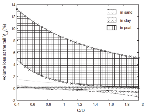
Figure 9. Volume loss at the tail in various soil when tunneling with D=6 m
