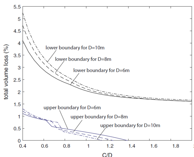
Figure 13. Total volume loss for tunnelling in sand
