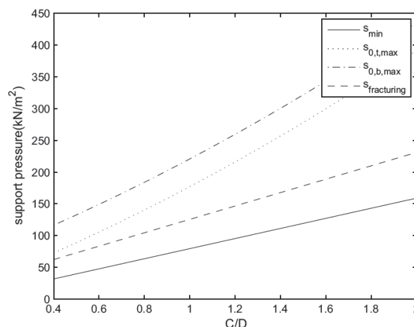
Figure 1. The range of support pressures at the tunnelling face of a tunnel with a diameter D=6 m in clay
