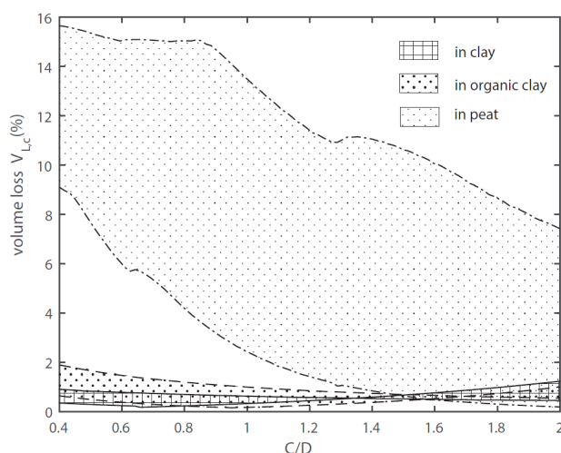
Figure 12. Volume loss due to consolidation V_{Lc} with a tunnel diameter D=6m in various soils
