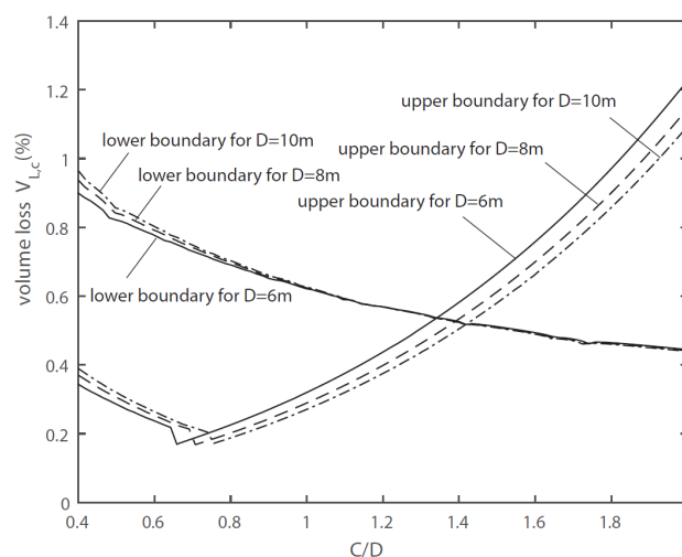
Figure 11. Volume loss due to consolidation V_{L,c} with different tunnel diameters in clay
