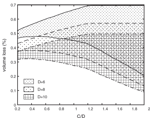
Figure 5. Volume loss along the shield in sand
