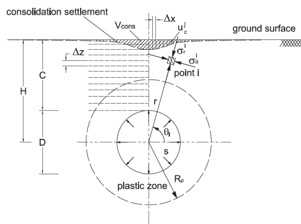
Figure 10. Soil stresses at the tail
