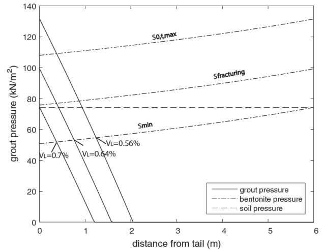
Figure 4. Grout pressures along a shield ( D=6 m) in clay.
