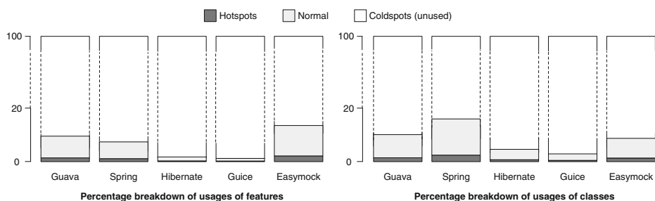
Fig. 8 Percentage breakdown of usage of features for each of the APIs
