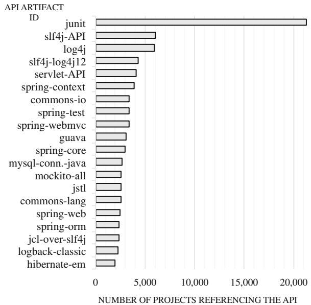
Fig. 1 Popularity of APIs referenced on Github
