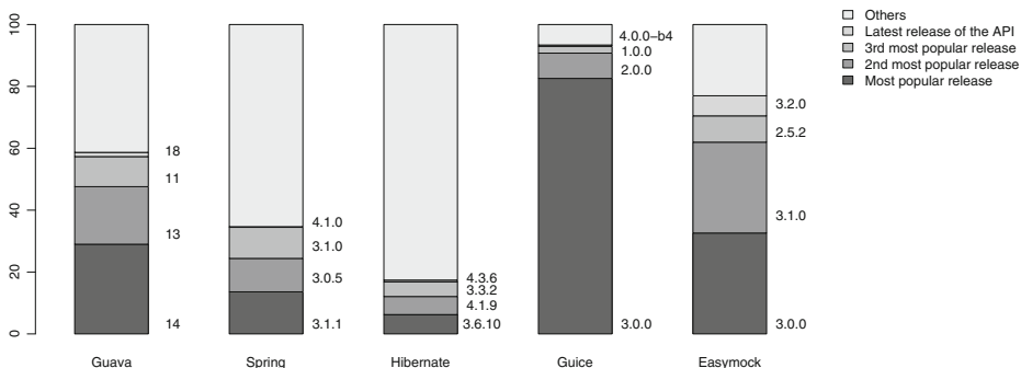
Fig. 5 Proportion of release adoption, split in the 3 most popular, the latest, and all the other releases, by API
