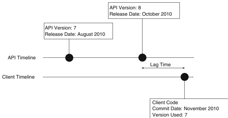
Fig. 3 An example of the lag time metric inspired by McDonnell et al. (2013)
