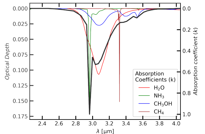
Fig. 11. Optical depth of the 3\ \mu\text{m} \text{H}_2\text{O} ice feature derived from the spectral flux density obtained from model 2 in Fig. 10. The optical depth is shown in dark gray thick line and the absorption coefficients of ice species that have a feature in the plotted wavelength range are shown as colored thin lines.
