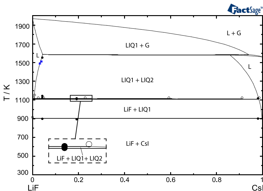
Fig. 10. The pseudo-binary phase diagram of the LiF–CsI joint. ● Data measured in this work *Evolution of the liquidus point during the different cycles. ○ Data by Margheritis et al. [29].
