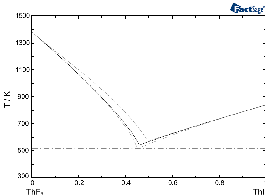
Fig. 6. Phase diagram of the \text{ThF}_4 - \text{ThI}_4 system estimated in this work. Dashed line: phase diagram calculated based on the \text{LiF} - \text{LiI} liquid excess parameters. Dashed-dotted line: phase diagram calculated based on the \text{CsF} - \text{CsI} liquid excess parameters.
