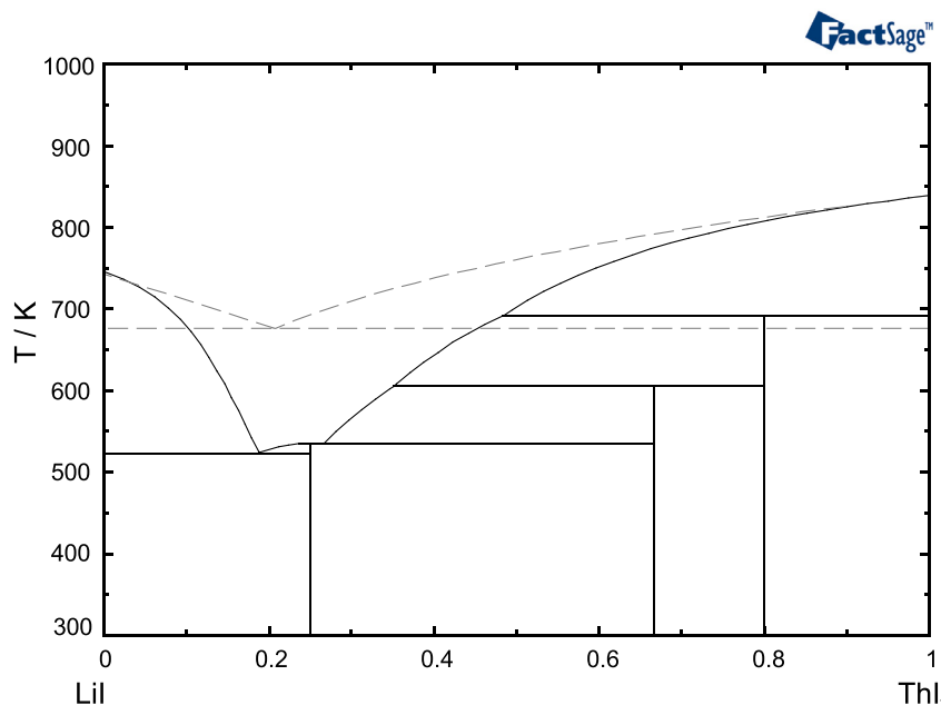
Fig. 7. Phase diagram of the \text{LiI} - \text{ThI}_4 system estimated in this work. Dashed line: Ideal behaviour without intermediate compounds.
