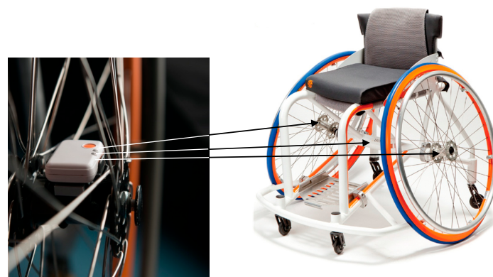
Figure 1. Sensor placement on the wheelchair, with one on each wheel axle and one on the frame camber bar (sensor picture by Marc Hollander Photography: www.marchollander.nl ).
