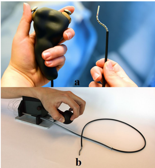
FIGURE 3. Prototypes of (a) the Sigma catheter with joystick control through thumb and index finger and (b) the Epsilon catheter with a handle that is an enlarged version of the tip.
