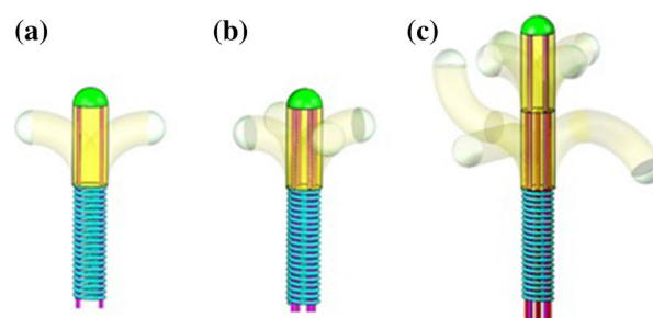
FIGURE 2. The concept of catheter steering with multiple segments explained in DOF, with (a) 1 DOF steering with one steerable segment, (b) 2 DOF steering with one steerable segment, and (c) 4 DOF steering with two steerable segments. Image adopted from Ref. 2.
