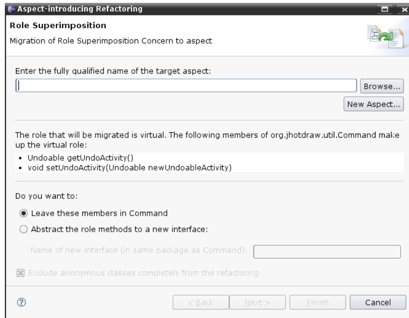
Figure 1: Providing input for virtual RSI refactoring
