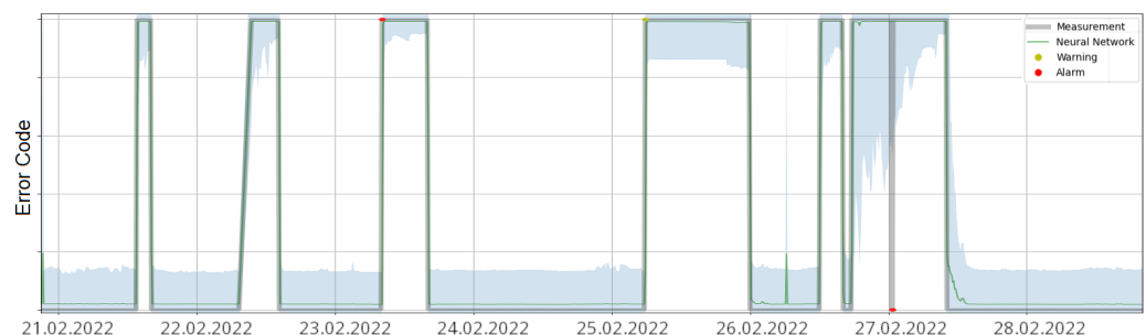
Figure 9. The direct modelling of the error codes leads to a model that can predict the gearbox failures very well as they happen but not in advance. This can be seen by the DNN (green line) following the error code (grey line) closely.
