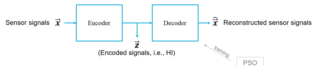
Figure 3. Architecture of the CAE.
