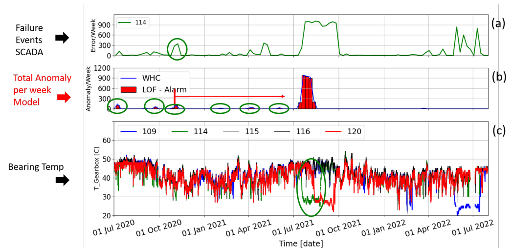
Figure 12. Error code from the SCADA data when the Turbine 114 indicates possible failures, with the data accumulated every week (a), Failure of Turbine 114 detected by WHC-LOF method with data accumulated every week (b), Time series of the bearing temperature of the five wind turbines where the green circle indicates that the bearing temperature drops when the Turbine 114 fails (c).
