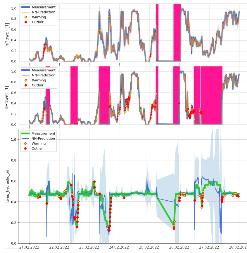
Figure 8. An example week for the WTG 120 (top) and 109 (middle) with several gearbox error codes. As can be seen for WTG 109, in some cases there is a accumulation of anomalies quite some time before the gearbox failure (21, 25, and 26 February 2022). On the other hand there is no anomaly accumulation before the 22 and especially the 23 February 2022. Furthermore, there is an anomaly accumulation at the 24 February 2022 with no following gearbox failure. Temperature of the hydraulic oil (bottom) is however spiking before the 22. The same week as for the WTG 109 is shown for the WTG 120. There is no significant anomaly accumulation on the 25 February 2022 and there is an accumulation on the 21 February 2022, where no gearbox failure is detected. nPower refers to normalised power, which is the power divided by the maximum observed power in the data set.
