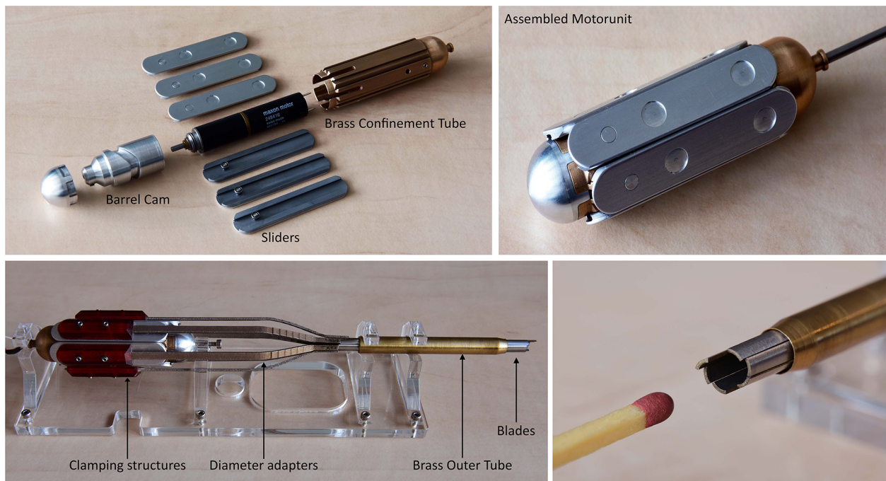
FIGURE 3 | Assembled prototype.
