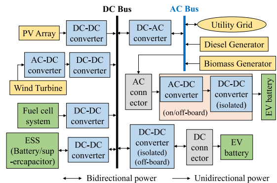
FIGURE 7. AC and DC-based architecture of HCS.
