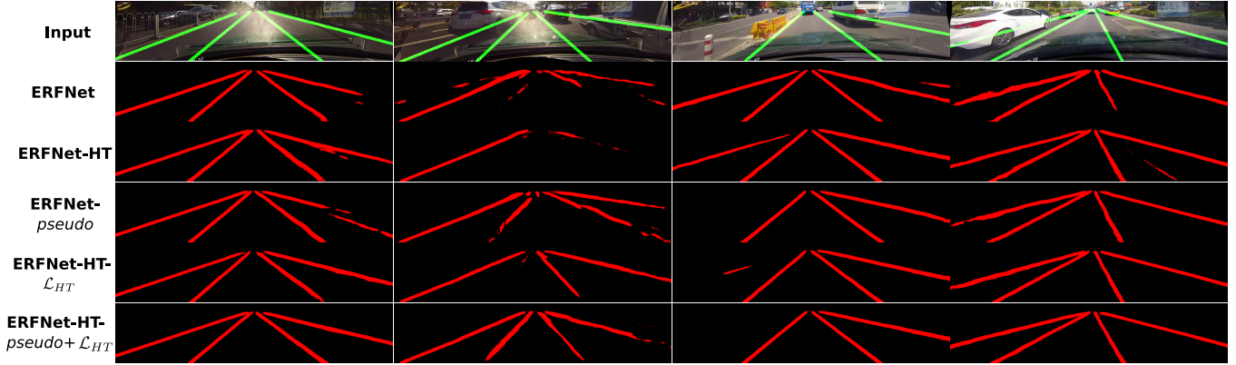
Fig. 2: Visualizations of predicted lanes on the CULane dataset. Only 10% annotated data is used for training. ERFNet-HT- pseudo + \mathcal{L}_{HT} performs better on challenging samples and better localizes lane boundaries. The inference speed of the ERFNet-HT is around 13 frames per second on a NVIDIA GTX1080Ti GPU.
