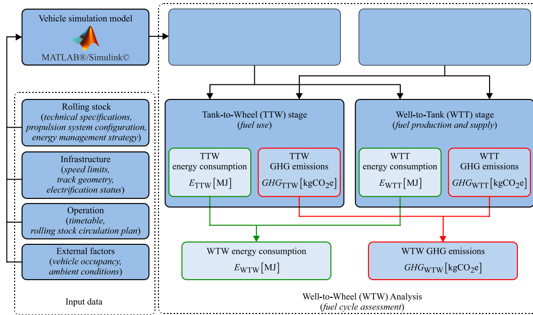
Fig. 1. Methodological framework for the assessment of Well-to-Wheel energy use and greenhouse gas emissions of regional trains.
