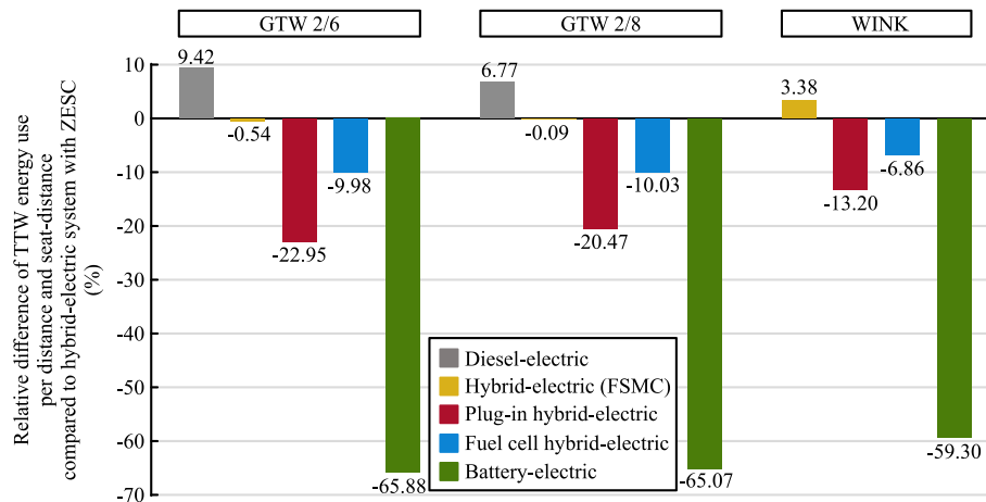
Fig. 10. Comparison of Tank-to-Wheel (TTW) energy use between alternative propulsion systems, based on hybrid-electric system with ZESC as a benchmark, and the overall mean values aggregated over alternative energy carriers.
