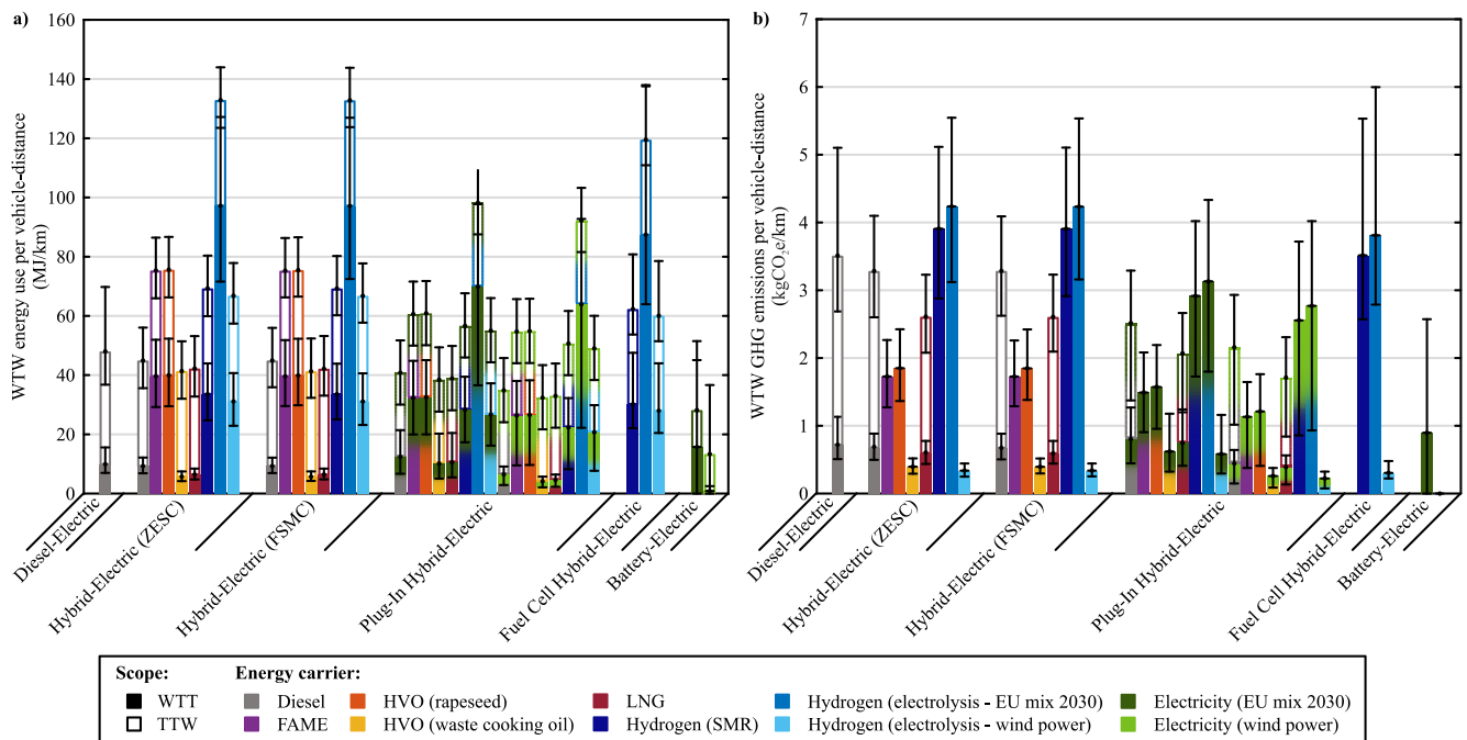
Fig. 13. Well-to-Tank (WTT), Tank-to-Wheel (TTW) and Well-to-Wheel (WTW) estimations of (a) energy use and (b) greenhouse gas (GHG) emissions per vehicle-distance for GTW 2/8 multiple unit vehicle.
