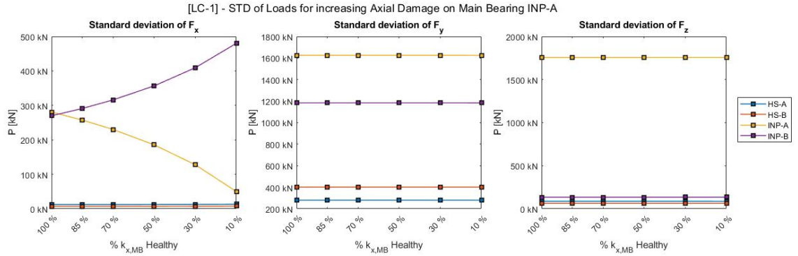
(b) Evolution of the standard deviation of forces for decreasing axial stiffness of MS bearing
