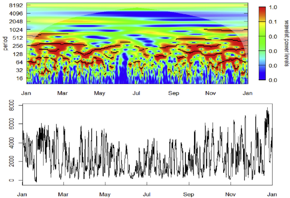
Figure 23: Wavelet Transform power Spectrum showing the most relevant coefficients shown in red and marked with a black line and below the reconstruction of the original signal filtered of noise using these significant coefficients [10]
