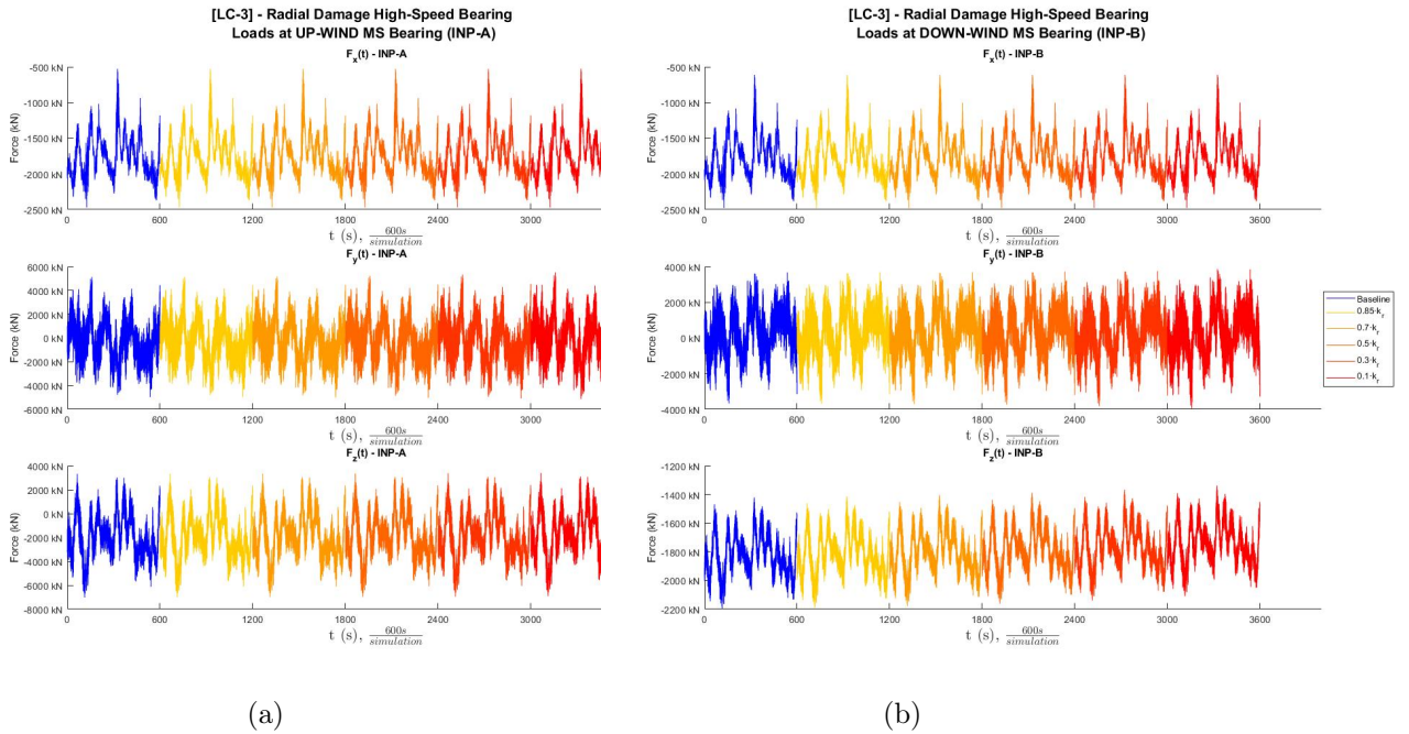
Figure 35: Evolution of F_x , F_y and F_z (a) at INP-A and (b) at INP-B for a radial damage occurring at HSS bearing HS-B ( LC3 )
