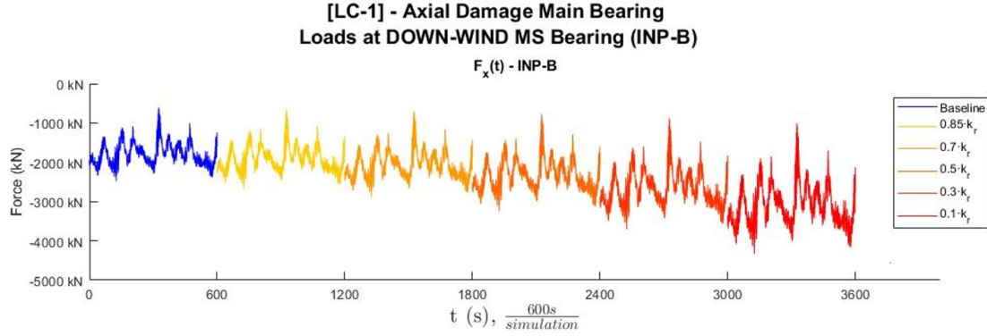
Figure 26: Evolution of F_x measured at INP-B for an axial damage occurring at bearing INP-A ( LC1 )
