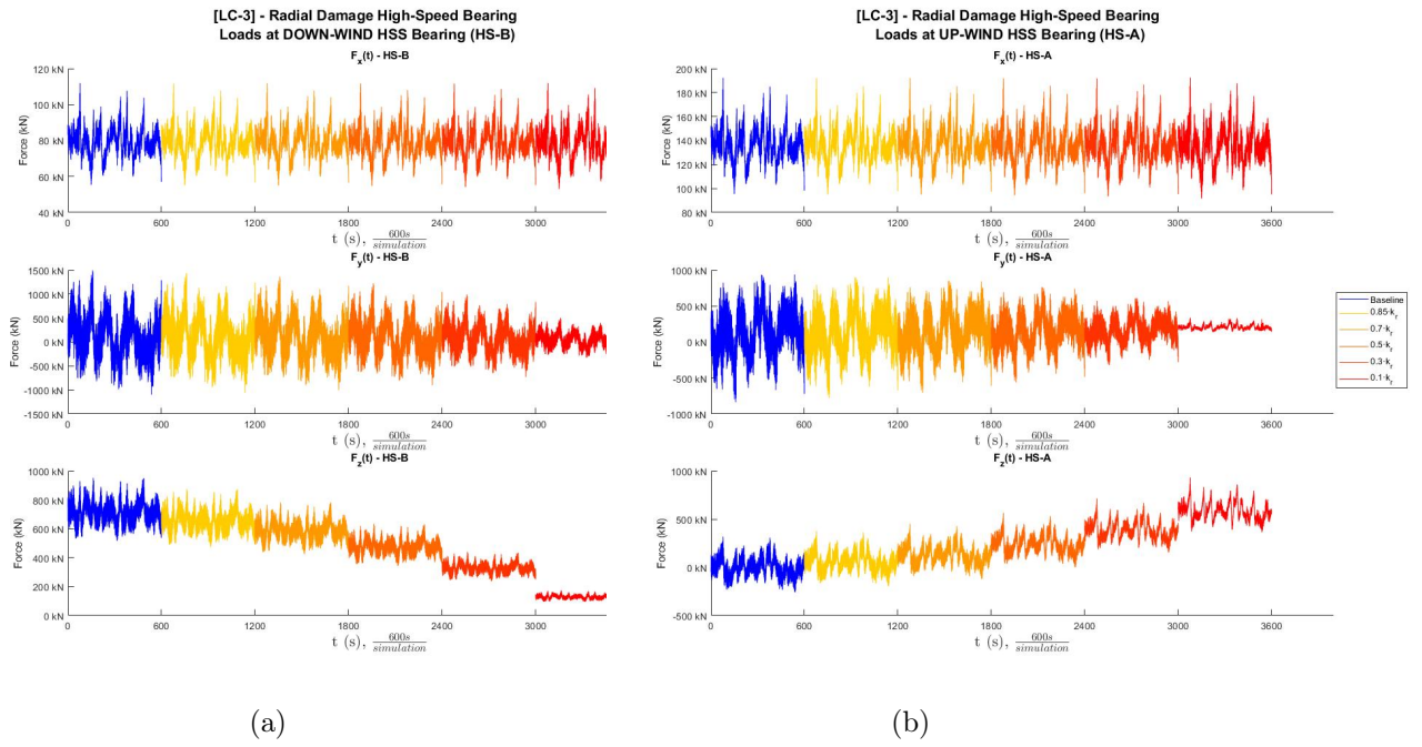
Figure 34: Evolution of F_x , F_y and F_z (a) at HS-B and (b) at HS-A for a radial damage occurring at HSS bearing HS-B ( LC3 )
