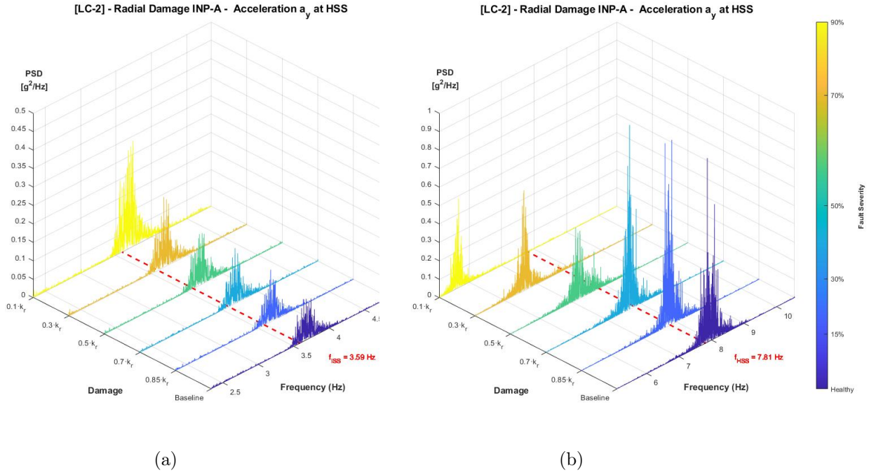
Figure 40: PSD of the acceleration signal \ddot{y} of the HSS showing (a) an increase of the energy content at f_{HSS} and (b) a variation of the magnitude and location of the energy content at f_{HSS} for LC2
