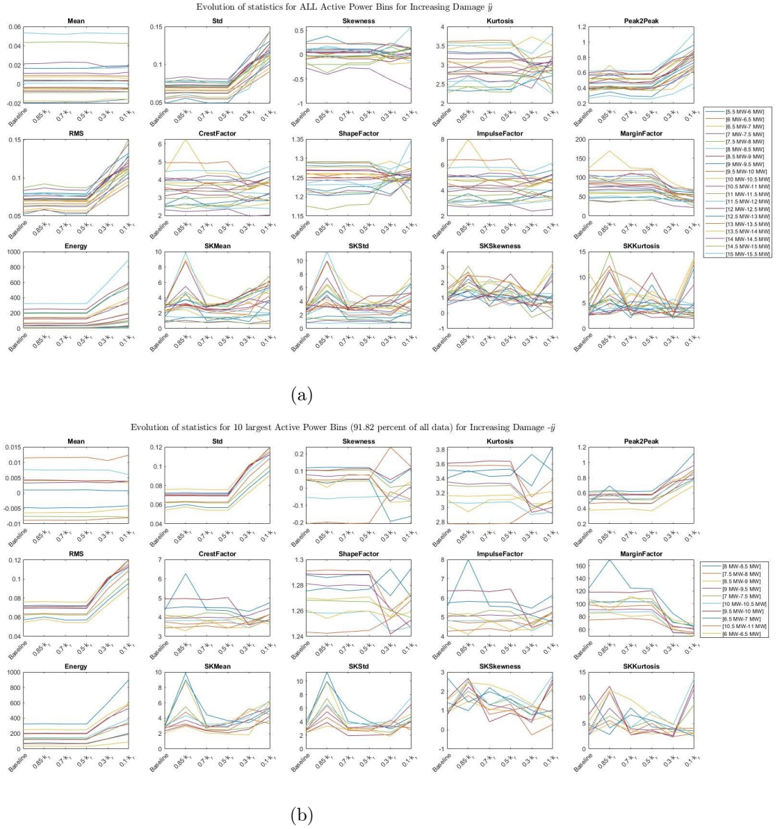
Figure 60: Evolution of statistical and spectral features of the MS acceleration \ddot{y} for load case LC1 shown (a) for all 20 power bins and (b) for 10 most populous power bins representing 91.8% of all measurements
