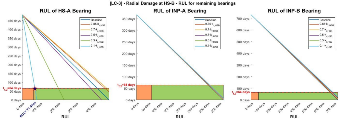
Figure 53: Predicted RUL of HS-A , INP-A and INP-B according to physics-based model for both failure thresholds for load case LC3
