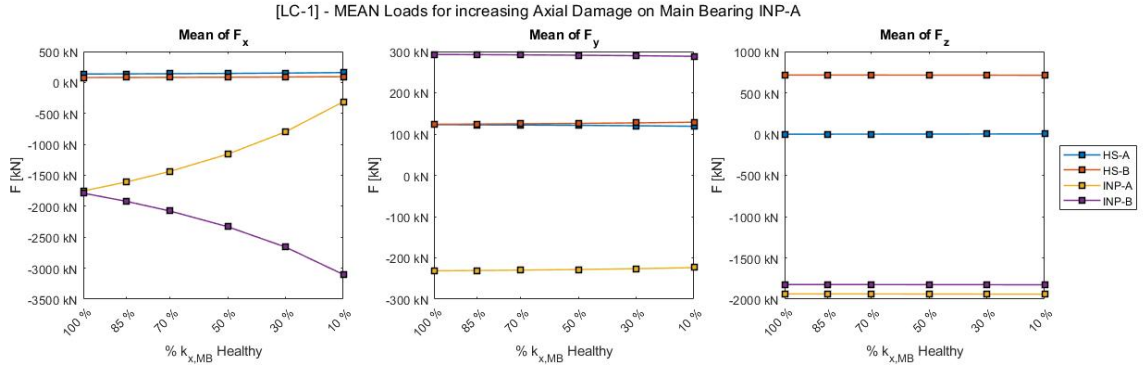
(a) Evolution of the mean value of forces for decreasing axial stiffness of MS bearing
