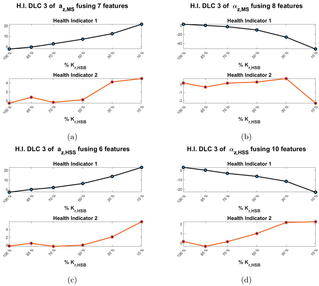
Figure 67: Potential health indicators (H.I) for \ddot{z} and \ddot{a}_z in the MS (a),(b) and HSS (c),(d) corresponding to LC3
