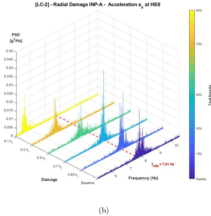
Figure 41: Evolution of PSD of \ddot{x} of HSS for LC2. (a) for a large frequency range and (b) for a frequency range in the surroundings of the HSS frequency f_{HSS}
