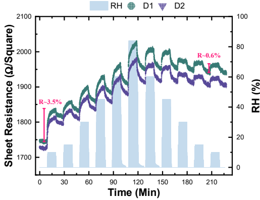
Fig. 3. MLG sheet resistance (left y-axis) of two devices based on MLG at different humidity steps (right y-axis). The two MLG strips devices are indicated by D1 and D2. The response at the first and last humidity steps is indicated in the plot.
