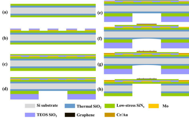
Fig. 1. The fabrication process of MLG strips integrated on a MHP. (a) Coating of the starting material with SiO 2 /SiNx stacking. (b) Mo heater patterning. (c) Isolation layer of the Mo heater electrodes and the sensing layer. (d) Hard mask patterning on the backside for the Si cavity under the MHP. (e) Partially open pads step prior to the MLG synthesis. (f) Fully opened micro-heaters pad after SiO 2 removal. (g) Cr/Au electrodes evaporation. (h) MLG on the MHP after backside SiO 2 /Si etching and Mo catalyst etching.
