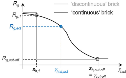
Figure 3. Continuous, rather than stepwise, elastic shear stiffness reduction factor as a function of the shear strain measure.
