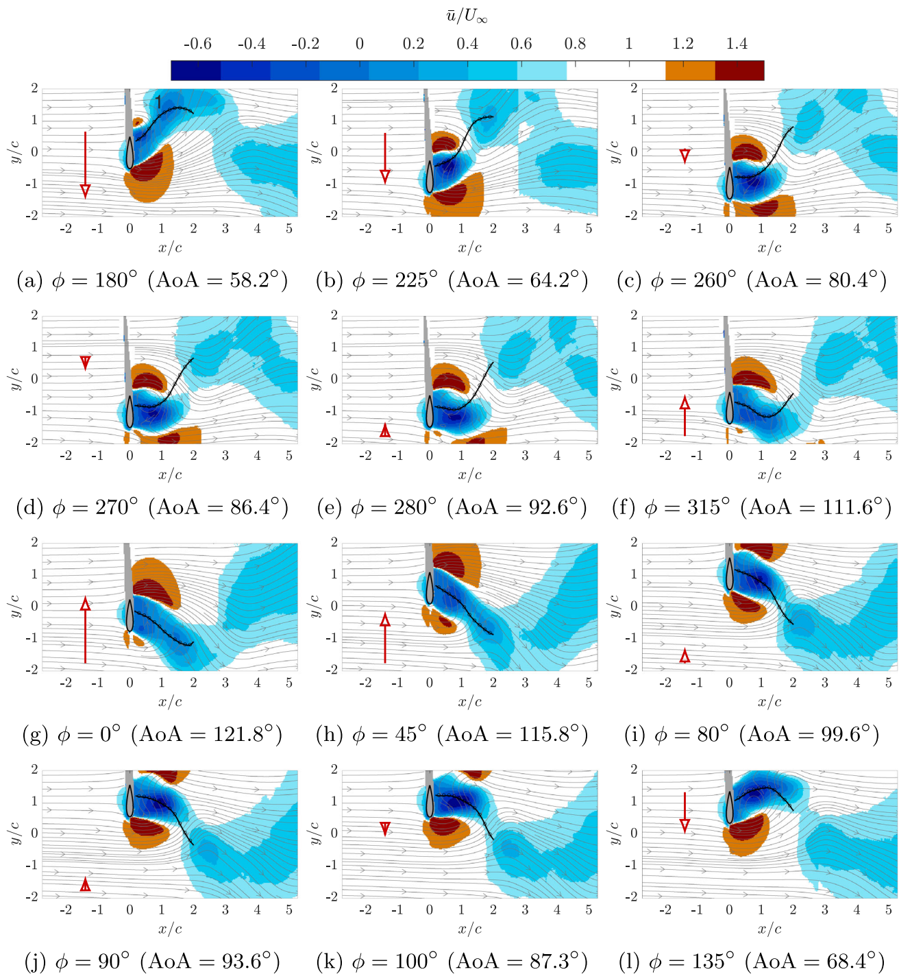
Fig. 11 Streamwise velocity field \bar{u}/U_\infty for k = 0.38 plunging case at all measured phases. The red arrow represents the scaled motion velocity \dot{h} . The wake center line is marked by the black circled line
