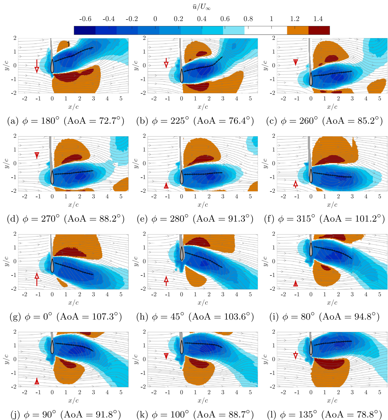
Fig. 7 Streamwise velocity field \bar{u}/U_\infty for k = 0.19 plunging case at all measured phases. The red arrow represents the scaled motion velocity \dot{h} . The wake center line is marked by the black dashed line
