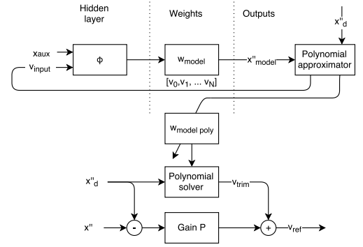
Figure 7. Inversion controller
