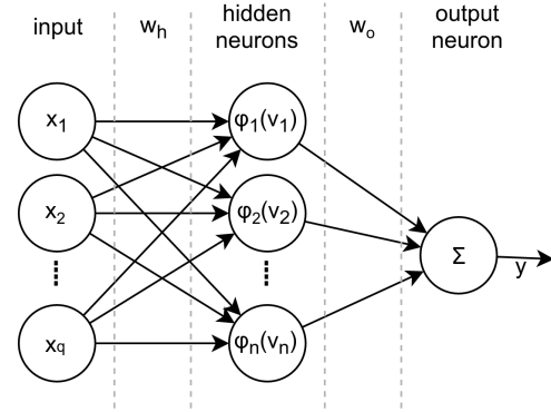
Figure 1. Neural net layout
