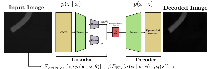
Fig. 2. A view of the overall neural architecture (from top left to bottom right). Thanks to the regularization imposed by the variational mechanism, the encoder can extract a one-dimensional smooth representation of the object configuration. Based on that, we show that a simple MLP architecture is sufficient to predict the evolution accurately in latent space from n past images. Finally, the prediction is passed through the decoder, yielding predicted images.
