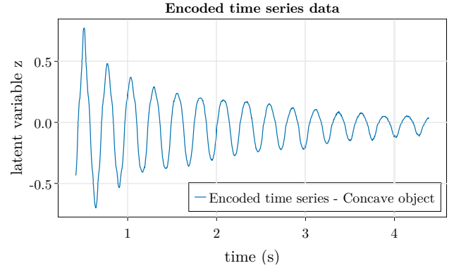
Fig. 9. Example of 4.5 seconds of video data encoded into the latent space via the AE with variational smoothing.
