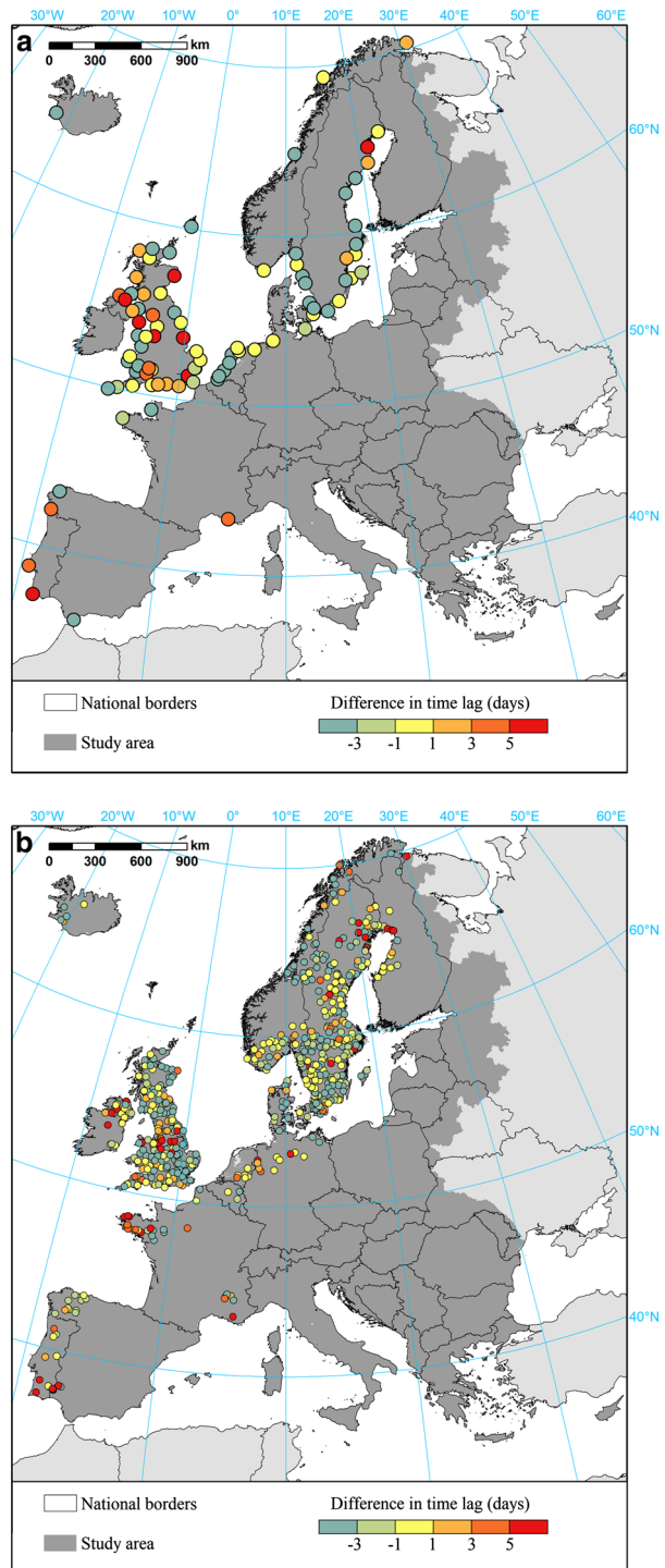
Fig. 7 Difference in the time lag in occurrence of storm surge events and a precipitation; b river discharges, that results in the highest value of the upper tail dependence coefficient (UTDC), between hindcast and observed data. The connections between river gauges and tide gauges from observations are preserved here for comparability with Fig. 5. The modelled and observed data were censored to a common series length
