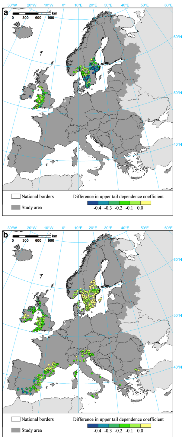
Fig. 8 Difference in upper tail dependence coefficient (UTDC) for the combination of storm surge events and river discharges, when 20% of significant wave height is added to the storm surge data, for a observed; b reanalysis data. The connections between river gauges and tide gauges from observations are preserved in (b) for comparability with (a)
