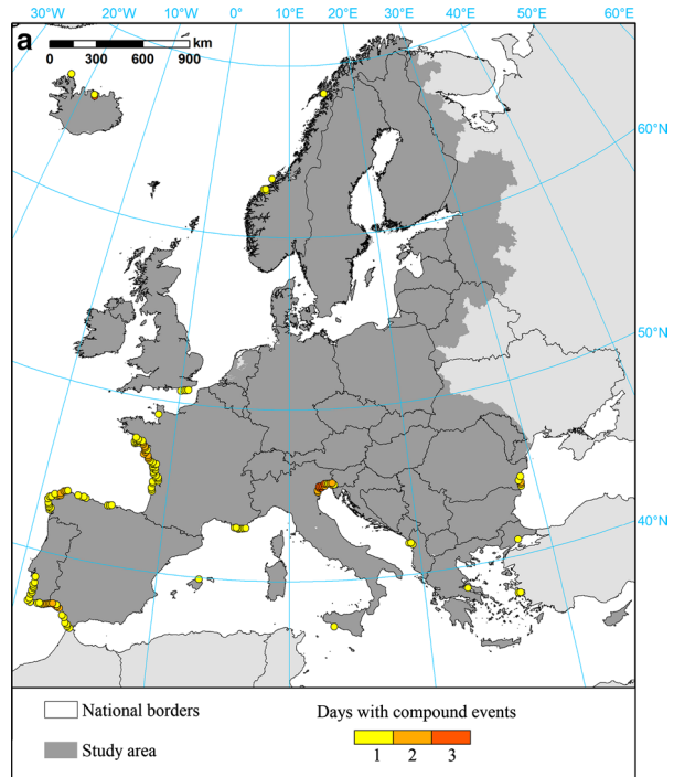
Fig. 4 Compound flood events identified in the reanalysis data, for the combination of storm surge events and a precipitation (1979–2014); b river discharges (1990–2013). The colours indicate the number of days with occurrence of compound events (some events lasted more than 1 day). A compound event is defined here as the occurrence of a storm surge event with a maximum of daily average height at least equal to a 5-year return period, during which (with an additional \pm 1 day window) daily precipitation or river discharge peaked at a value at least equal to a 5-year return period
