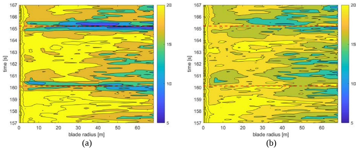
Figure 4. Ten-second time window of the turbulent inflow with a mean wind speed of 16 m/s along the blade length, for (a) an downwind configuration, and (b) an upwind configuration. The colouring indicates the flow velocity and the red dashed lines indicate the time instances of the blade passing the centre line of the tower.
