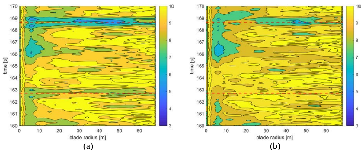
Figure 3. Ten-second time window of the turbulent inflow with a mean wind speed of 7 m/s along the blade length, for (a) an downwind configuration, and (b) an upwind configuration. The colouring indicates the flow velocity and the red dashed lines indicate the time instances of the blade passing the centre line of the tower.
