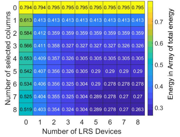
Fig. 10. Energy consumed in an 8 \times 8 array during MAC operation, as function of number of selected columns and LRS devices.
