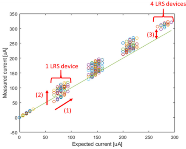
Fig. 9. VMM using RRAM crossbar array: Current measurements for a single column in a 8 \times 8 array.
