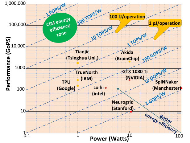
Fig. 11. Illustration of energy efficiency for various hardware and CIM energy-efficiency potential [75].
