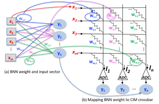
Fig. 7. Mapping of BNN weights to crossbar array illustrating weight mapping and MAC operation for each neuron.
