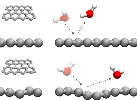
FIG. 2. Schematic depiction of a water molecule interacting with rigid (top) and flexible (bottom) wall surfaces. The deflection of wall atoms in the flexible wall may cause a reduction in solid-fluid friction and result in a faster fluid flow.
