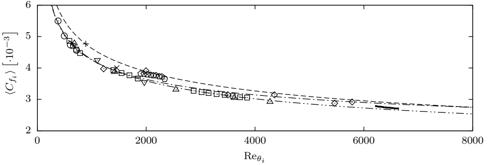
Figure 5: Incompressible skin-friction distribution. (—) Present LES ( \mathcal{G}^2 ), (----) Blasius, (-·-·-) Kármán-Schoenherr (both adopted from Hopkins & Inouye (1971)), (-·-·-·) Smits et al. (1983), ( \square ) Pirozzoli & Bernardini (2011), ( \odot ) Komminaho & Skote (2002), ( \triangle ) Schlatter & Örlü (2010), ( \nabla ) Simens et al. (2009), ( \diamond ) Pirozzoli et al. (2004), ( \times ) Maeder et al. (2001), (+) Guarini et al. (2000), ( \diamond ) Coles (1953) (CAT5301, from Fernholz & Finley (1977))
