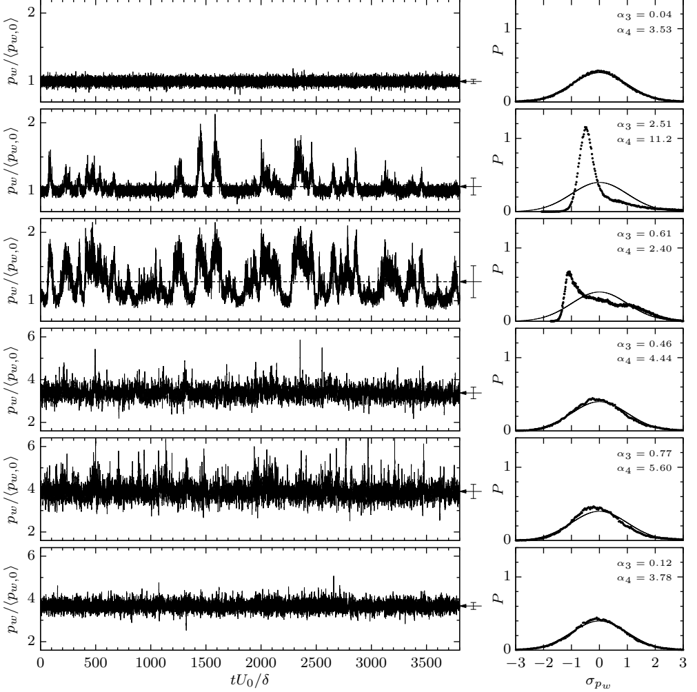
Figure 15: Wall-pressure signals (left) and corresponding normalised probability density distributions (right) evaluated at (x-x_{imp})/\delta = \{-17.74, -11.66, -11.34, 4.25, 6.61, 17.18\} . Refer to the text and figure 14 for a physical interpretation of the wall-pressure positions. The mean wall-pressure is indicated by a horizontal dashed line. Arrows together with vertical bars indicate the mean wall-pressure and its standard deviation. Values of skewness \alpha_3 and flatness \alpha_4 coefficients and a Gaussian distribution are included for reference.
