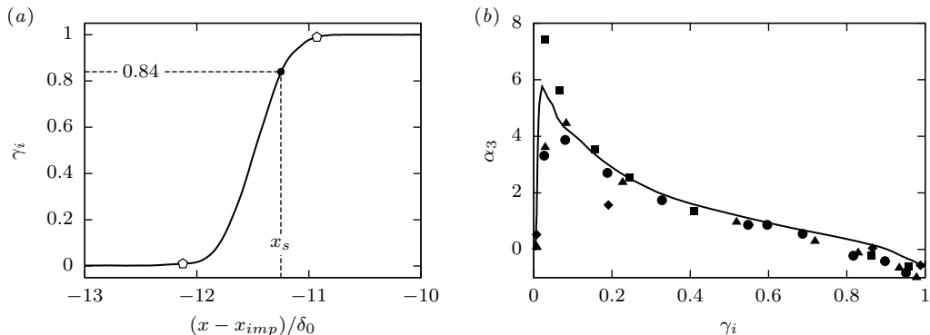
Figure 16: (a) Streamwise intermittency distribution \gamma_i(x) . The mean separation location x_s is indicated. ( \circ ) highlight 1% and 99% intermittency boundaries and define the intermittent lengthscale L_i = 1.2\delta_0 . (b) Skewness coefficient \alpha_3 as a function of intermittency \gamma_i . (—) LES. Symbols represent experimental data from Dolling & Or (1985) for a compression ramp flow at a Mach number of Ma = 2.9 and a Reynolds number of Re_{\delta_0} = 1.43 \cdot 10^6 with wedge angles ( \blacklozenge ) \vartheta = 12^\circ (attached flow), ( \bullet ) \vartheta = 16^\circ (incipient separation), ( \blacktriangle ) \vartheta = 20^\circ (separated flow) and ( \blacksquare ) \vartheta = 24^\circ (separated flow).
