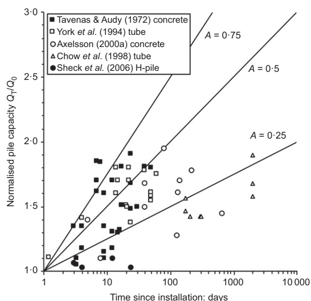
Fig. 1. Case histories of pile set-up in sandy soil (after Zhang & Wang, 2014)
