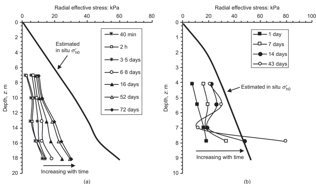
Fig. 2. Radial stresses measured during ageing of pre-cast driven concrete piles from (a) Hunters Point (Ng et al. , 1988) and (b) Fittja Straits (Axelsson, 2000a)
