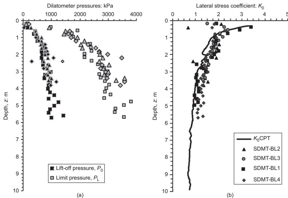
Fig. 5. (a) Dilatometer lift and limit pressures and (b) estimated coefficient of earth pressure at rest, K_0 values for Blessington
