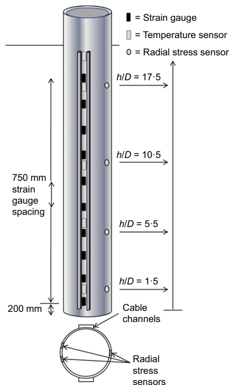
Fig. 6. Layout of pile instrumentation
