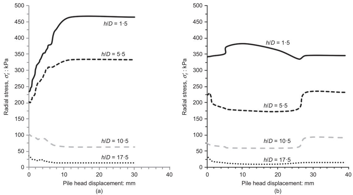
Fig. 13. Radial stress during load test on (a) pile S6 at 116 days and (b) pile S7 at 4 days
