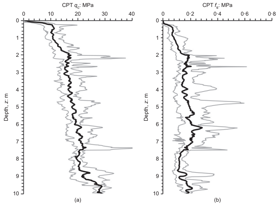
Fig. 4. (a) CPT cone resistance; (b) CPT sleeve friction at Blessington. The grey lines represent minimum and maximum values, the black lines represent the average values
