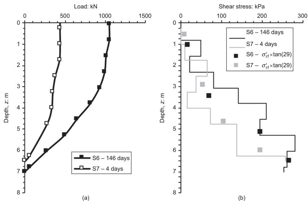
Fig. 14. Comparison of (a) load measured and (b) distribution of shear stress on piles S6 and S7
