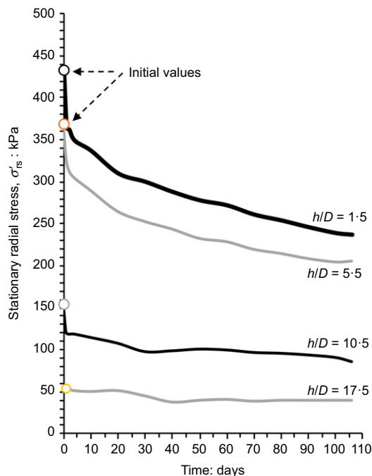
Fig. 10. Changes in radial stress during ageing of pile S6
