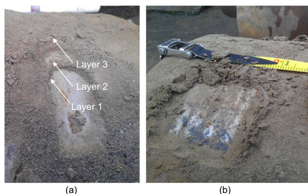
Fig. 15. Photographs of cemented sand crust adhered to pile S6 following extraction: (a) cemented sand crust on pile with distinct layers; (b) difficulty removing layer 1
