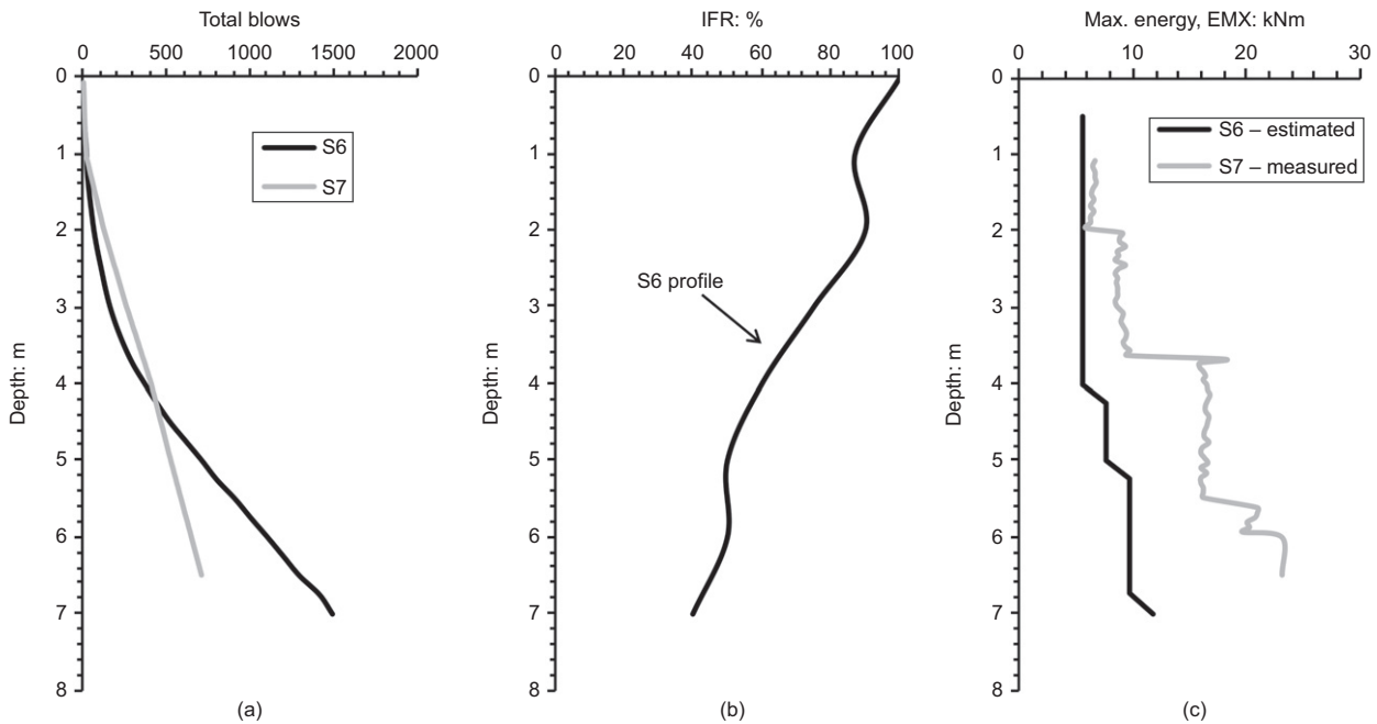
Fig. 7. (a) Total blows; (b) incremental filling ratio during pile installation; (c) energy measurements during pile installation
