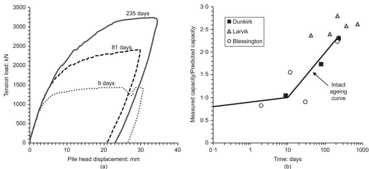
Fig. 3. (a) Ageing load test response at Dunkirk (after Jardine et al. , 2006). (b) Variation of normalised capacity with time
