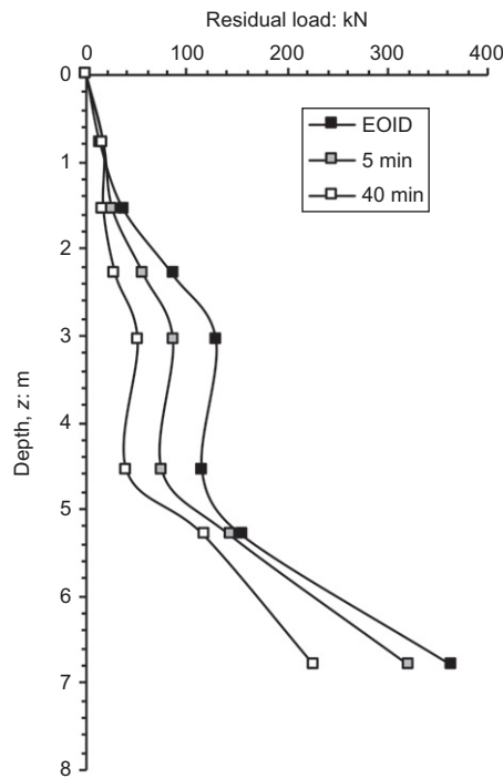
Fig. 9. Residual loads measured on pile S6 using strain gauges. EOID, end of installation
