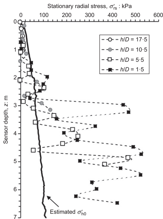
Fig. 8. Stationary radial stresses measured during driving pause periods for pile S6
