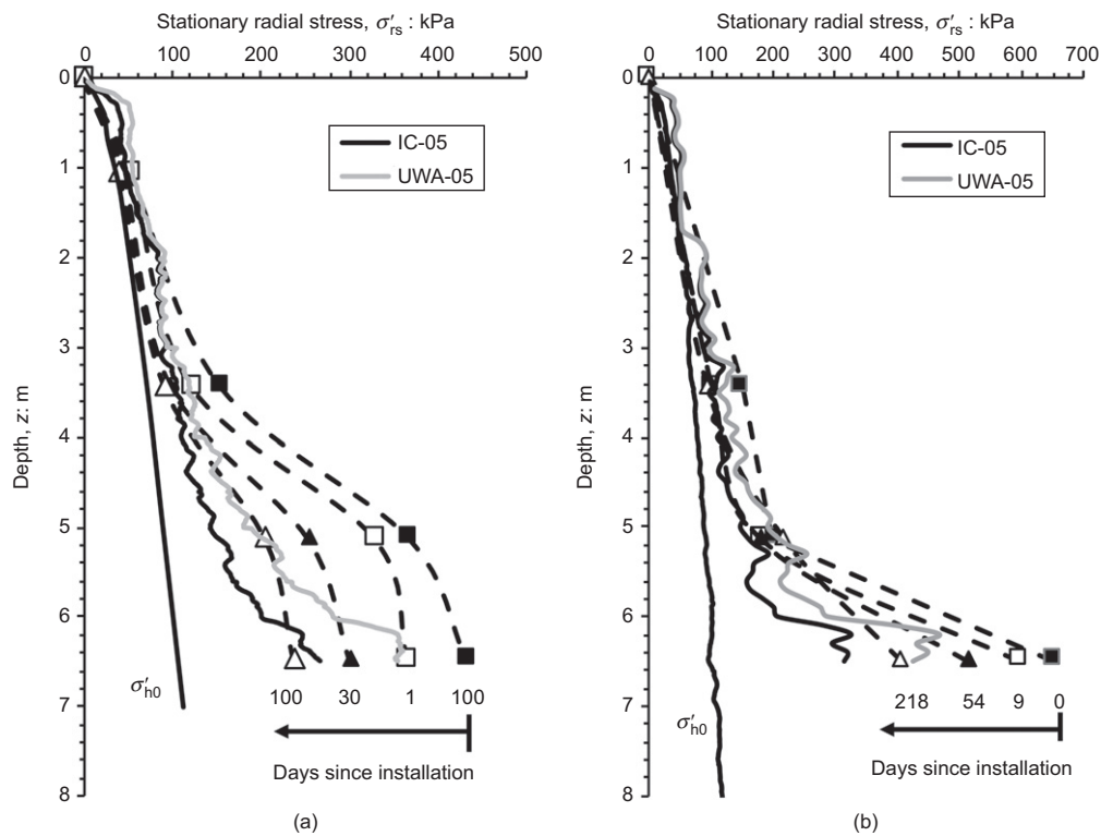
Fig. 11. Radial stress profiles measured over ageing period: (a) from pile S6; (b) from pile S5
