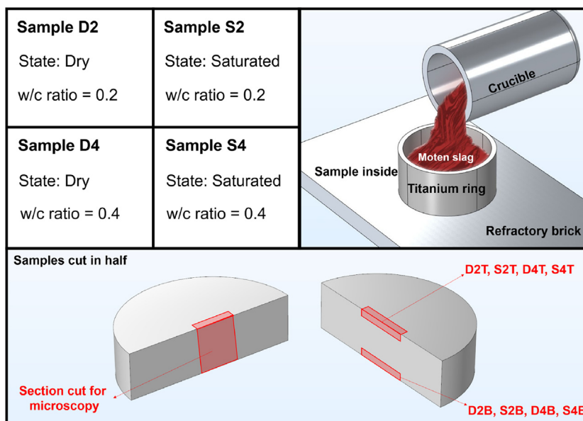
Fig. 1. Top left: Naming convention of samples. Top right: Sketch of thermal shock experiment. Bottom: Location of analysed parts in each sample.
