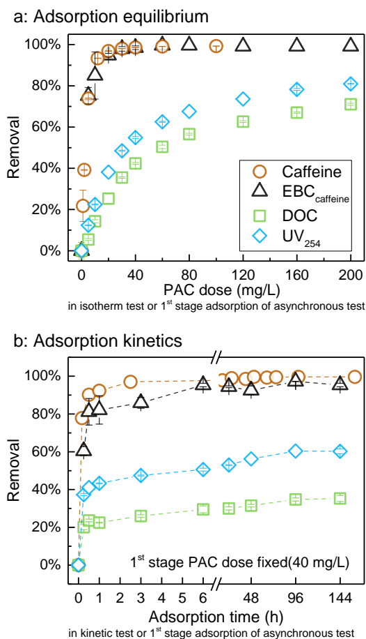
Figure 6 The removal of DOM competitor (fictive-EBC, and sum parameters including DOC and UV_{254} ) in the first stage of DOM-OMP asynchronous adsorption as compared to removal of caffeine (data extracted from OMP-spiked isotherm/kinetic test) at (a) adsorption equilibrium with various first stage PAC doses; (b) adsorption kinetics with PAC_{40\text{mg/L}} pretreatment in the first stage adsorption. Note that second stage adsorption were all in 7 d; EBC removal calculation was based on fixed K_{F,EBC} ( 21.84 \text{ (nmol/mg)}/(\text{nmol/L})^{1/n} ) and 1/n_{EBC} (0.69).
