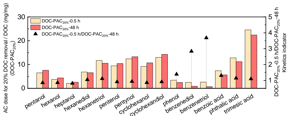
Figure S8 mDOM adsorbability at non-equilibrium adsorption (DOC-PAC 20% -0.5 h) and equilibrium adsorption (DOC-PAC 20% -48 h). The ratio of DOC-PAC 20% -0.5 h and DOC-PAC 20% -48 h calculated as a kinetic indicator to evaluate how far mDOM reaches adsorption equilibrium.
