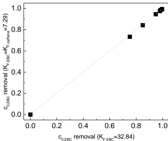
Figure S5 Comparison of c_{0,EBC} removal with different K_{F,EBC} values (unit: (nmol/mg)/(nmol/L) ^{1/n} ) applied. Reference line (grey) for the identical c_{0,EBC} removal.
