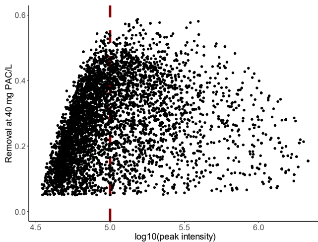
Figure S4 Percentage removal by PAC_{40mg/L} treatment vs. peak intensity (in log scale) of molecular formulas. The threshold of peak intensity ( >10^5 ) for the semi-quantitative analysis indicated (red dashed line).
